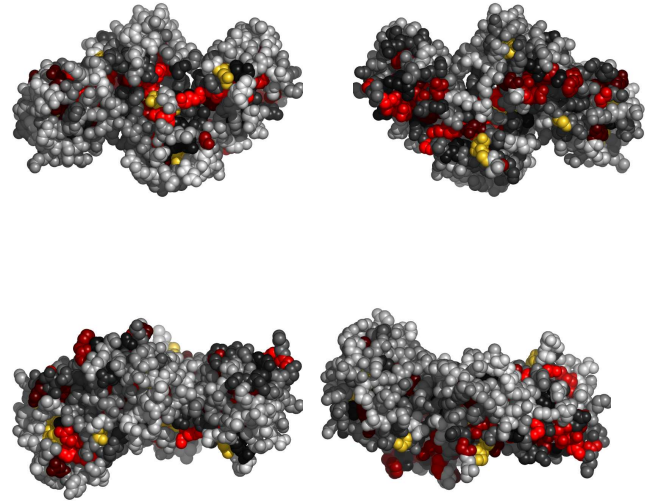
Fig. 2. Residues 164-318 in laowA colored by their relative importance. (See Appendix, Fig.8, for the coloring scheme.)
