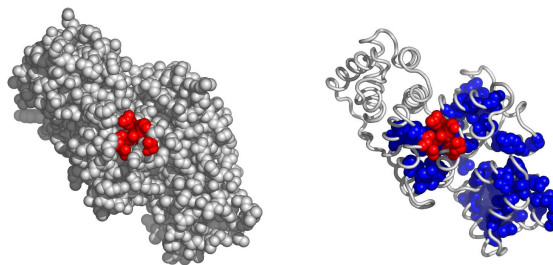
Fig. 6. Another possible active surface on the chain 1aowA. The larger cluster it belongs to is shown in blue.
