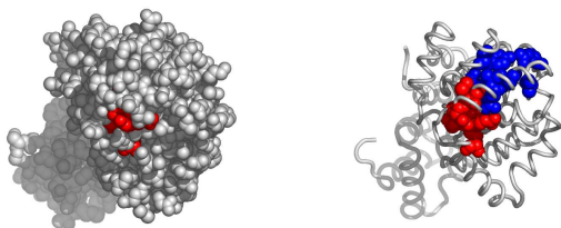
Fig. 7. Another possible active surface on the chain 1aowA. The larger cluster it belongs to is shown in blue.
