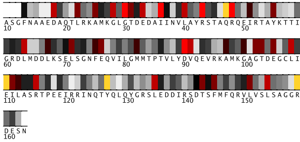
Fig. 1. Residues 10-163 in laowA colored by their relative importance. (See Appendix, Fig.8, for the coloring scheme.)
