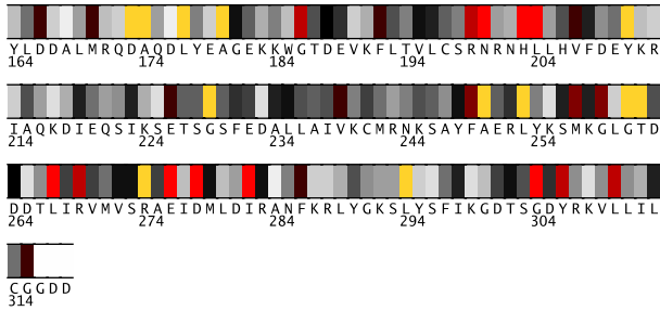
Fig. 2. Residues 164-318 in laowA colored by their relative importance. (See Appendix, Fig.8, for the coloring scheme.)
