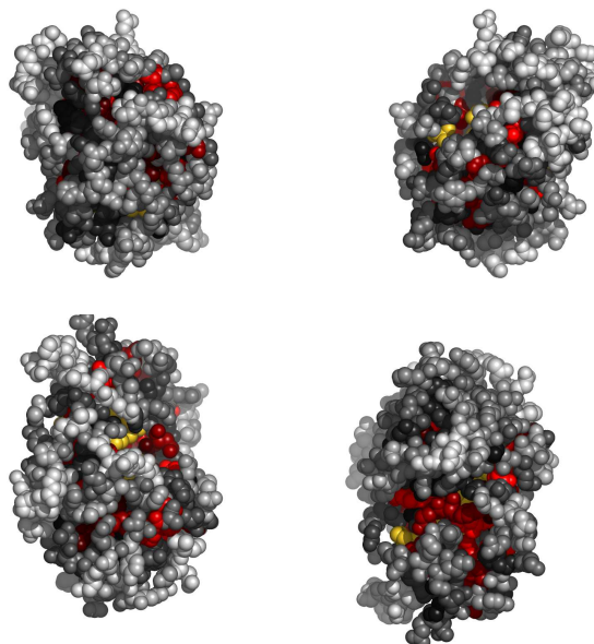
Fig. 3. Residues in 1apgA, colored by their relative importance. Clockwise: front, back, top and bottom views.
