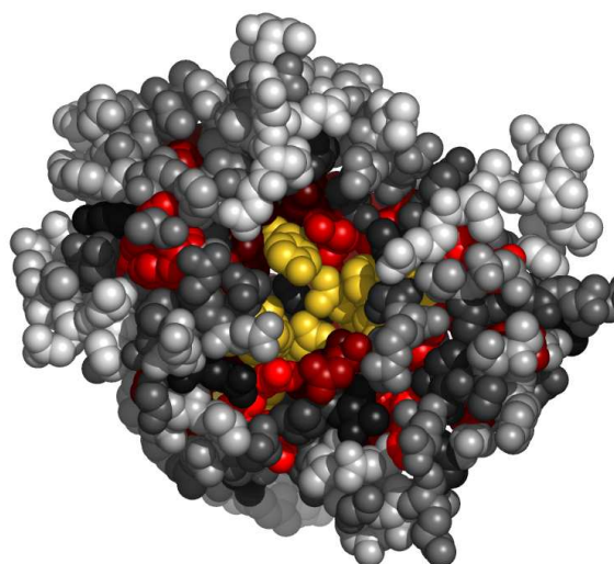
Fig. 5. Residues in lapgA , at the interface with DNA ( lapgD ), colored by their relative importance. DNA is colored green. (See Appendix for the coloring scheme for the protein chain lapgA .)
