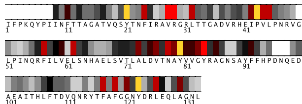
Fig. 1. Residues 1-133 in 1apgA colored by their relative importance. (See Appendix, Fig.7, for the coloring scheme.)
