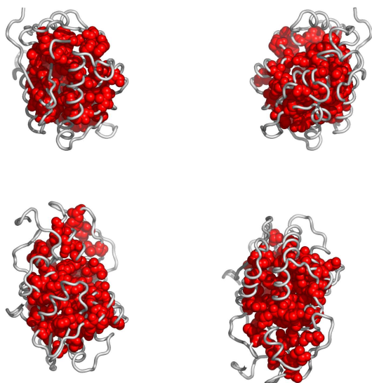
Fig. 4. Residues in 1apgA, colored according to the cluster they belong to: red, followed by blue and yellow are the largest clusters (see Appendix for the coloring scheme). Clockwise: front, back, top and bottom views. The corresponding Pymol script is attached.
