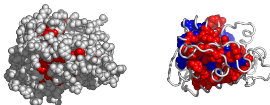
Fig. 6. A possible active surface on the chain lapgA . The larger cluster it belongs to is shown in blue.
