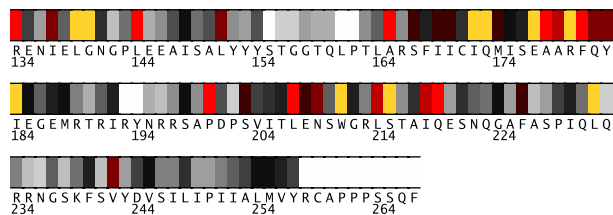
Fig. 2. Residues 134-267 in 1apgA colored by their relative importance. (See Appendix, Fig.7, for the coloring scheme.)
