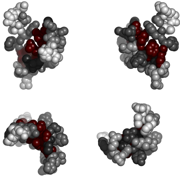
Fig. 2. Residues in laphB, colored by their relative importance. Clockwise: front, back, top and bottom views.
