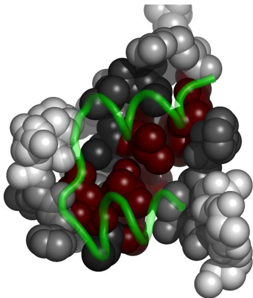
Fig. 4. Residues in laphB, at the interface with laphA, colored by their relative importance. laphA is shown in backbone representation (See Appendix for the coloring scheme for the protein chain laphB.)
