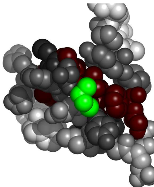
Fig. 5. Residues in laphB, at the interface with 1,2-dichloroethane, colored by their relative importance. The ligand (1,2-dichloroethane) is colored green. Atoms further than 30 Å away from the geometric center of the ligand, as well as on the line of sight to the ligand were removed. (See Appendix for the coloring scheme for the protein chain laphB.)
