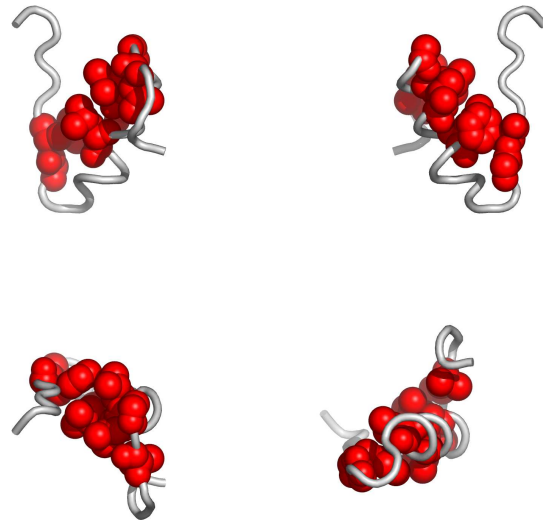
Fig. 2. Residues in laphB, colored by their relative importance. Clockwise: front, back, top and bottom views.
