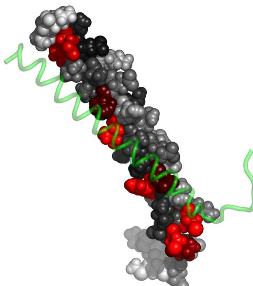
Fig. 5. Residues in 1aq5A, at the interface with 1aq5B, colored by their relative importance. 1aq5B is shown in backbone representation (See Appendix for the coloring scheme for the protein chain 1aq5A.)
