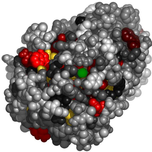
Fig. 5. Residues in 1aqhA, at the interface with chloride ion, colored by their relative importance. The ligand (chloride ion) is colored green. Atoms further than 30Å away from the geometric center of the ligand, as well as on the line of sight to the ligand were removed. (See Appendix for the coloring scheme for the protein chain 1aqhA.)
