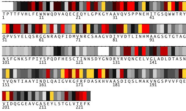
Fig. 1. Residues 1-224 in IaqhA colored by their relative importance. (See Appendix, Fig.8, for the coloring scheme.)
