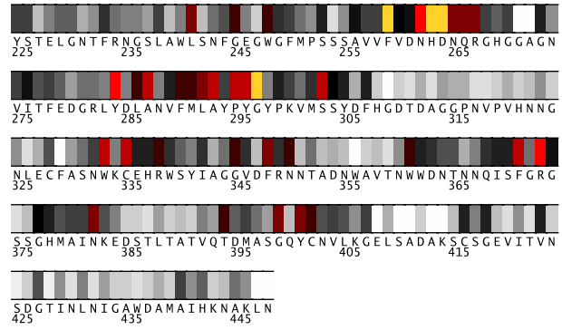
Fig. 2. Residues 225-448 in IaqhA colored by their relative importance. (See Appendix, Fig.8, for the coloring scheme.)
