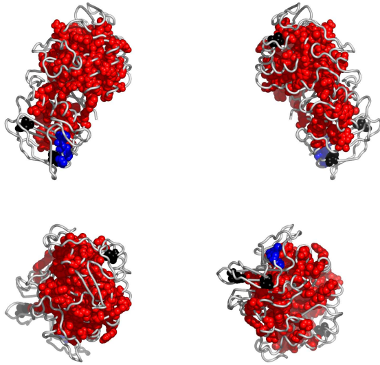
Fig. 4. Residues in 1aqhA, colored according to the cluster they belong to: red, followed by blue and yellow are the largest clusters (see Appendix for the coloring scheme). Clockwise: front, back, top and bottom views. The corresponding Pymol script is attached.
