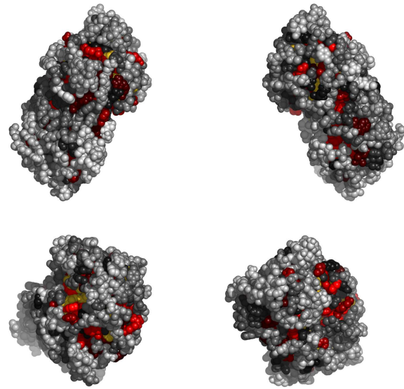
Fig. 2. Residues 225-448 in IaqhA colored by their relative importance. (See Appendix, Fig.8, for the coloring scheme.)
