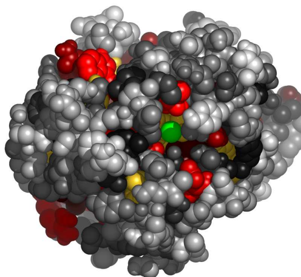
Fig. 6. Residues in 1aqhA, at the interface with calcium ion, colored by their relative importance. The ligand (calcium ion) is colored green. Atoms further than 30Å away from the geometric center of the ligand, as well as on the line of sight to the ligand were removed. (See Appendix for the coloring scheme for the protein chain 1aqhA.)
