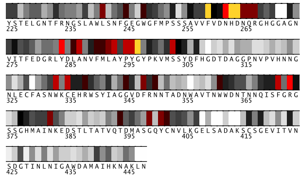
Fig. 2. Residues 225-448 in 1aqaA colored by their relative importance. (See Appendix, Fig.9, for the coloring scheme.)
