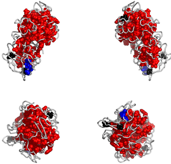
Fig. 4. Residues in 1aqmA, colored according to the cluster they belong to: red, followed by blue and yellow are the largest clusters (see Appendix for the coloring scheme). Clockwise: front, back, top and bottom views. The corresponding Pymol script is attached.
