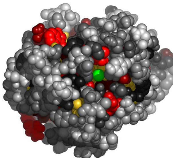
Fig. 6. Residues in 1aqmA, at the interface with calcium ion, colored by their relative importance. The ligand (calcium ion) is colored green. Atoms further than 30Å away from the geometric center of the ligand, as well as on the line of sight to the ligand were removed. (See Appendix for the coloring scheme for the protein chain 1aqmA.)
