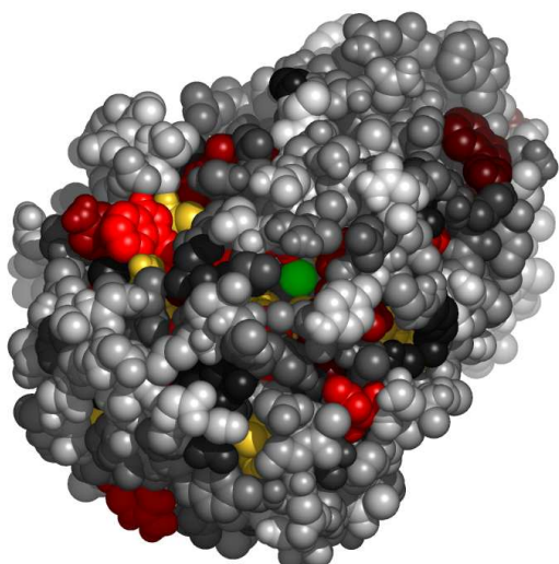
Fig. 5. Residues in 1aqmA, at the interface with chloride ion, colored by their relative importance. The ligand (chloride ion) is colored green. Atoms further than 30Å away from the geometric center of the ligand, as well as on the line of sight to the ligand were removed. (See Appendix for the coloring scheme for the protein chain 1aqmA.)
