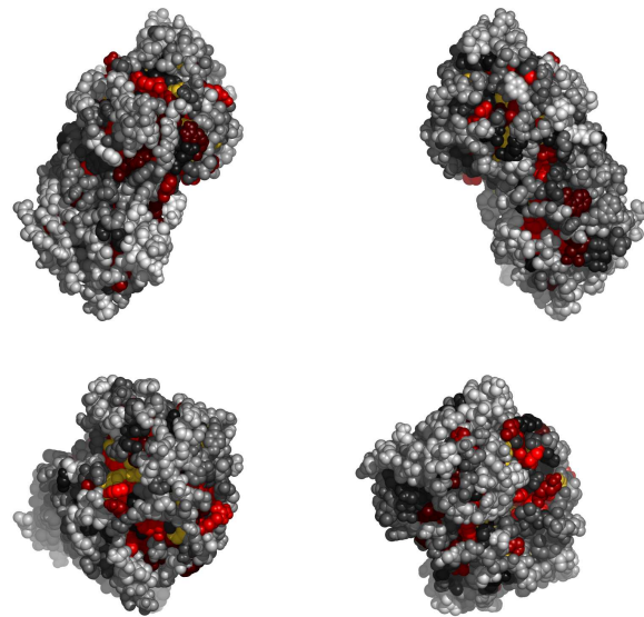
Fig. 2. Residues 225-448 in 1aqaA colored by their relative importance. (See Appendix, Fig.9, for the coloring scheme.)
