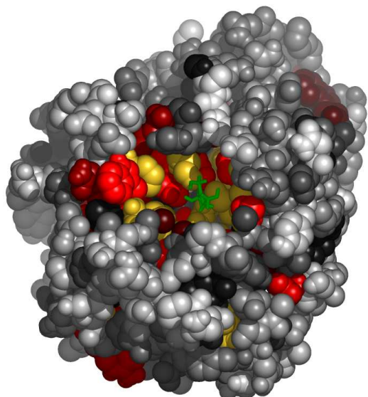
Fig. 7. Residues in 1aqmA, at the interface with TRS, colored by their relative importance. The ligand (TRS) is colored green. Atoms further than 30Å away from the geometric center of the ligand, as well as on the line of sight to the ligand were removed. (See Appendix for the coloring scheme for the protein chain 1aqmA.)
