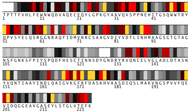
Fig. 1. Residues 1-224 in 1aqaA colored by their relative importance. (See Appendix, Fig.9, for the coloring scheme.)
