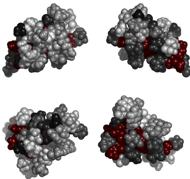
Fig. 2. Residues in latxA, colored by their relative importance. Clockwise: front, back, top and bottom views.
