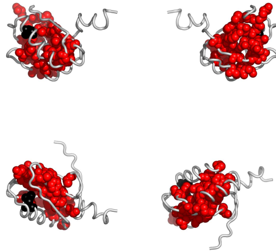
Fig. 3. Residues in laudA, colored according to the cluster they belong to: red, followed by blue and yellow are the largest clusters (see Appendix for the coloring scheme). Clockwise: front, back, top and bottom views. The corresponding Pymol script is attached.
