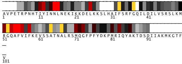
Fig. 1. Residues 1-101 in laudA colored by their relative importance. (See Appendix, Fig.6, for the coloring scheme.)
