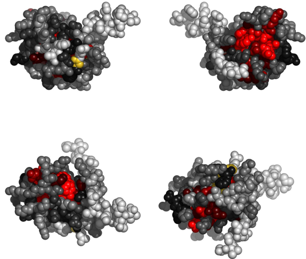
Fig. 2. Residues in laudA, colored by their relative importance. Clockwise: front, back, top and bottom views.
