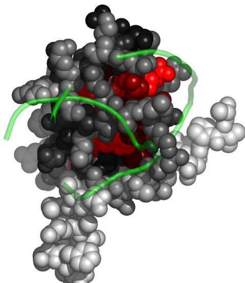
Fig. 4. Residues in laudA, at the interface with RNA (laudB), colored by their relative importance. RNA is colored green. (See Appendix for the coloring scheme for the protein chain laudA.)
