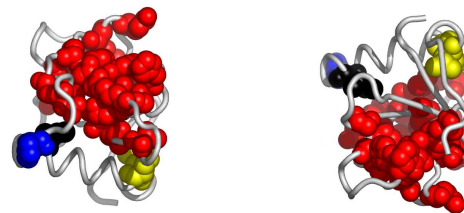
Fig. 3. Residues in 1ay7A, colored according to the cluster they belong to: red, followed by blue and yellow are the largest clusters (see Appendix for the coloring scheme). Clockwise: front, back, top and bottom views. The corresponding Pymol script is attached.
