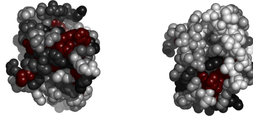
Fig. 2. Residues in 1ay7A, colored by their relative importance. Clockwise: front, back, top and bottom views.
