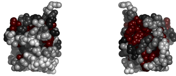
Fig. 1. Residues 1-96 in 1ay7A colored by their relative importance. (See Appendix, Fig.6, for the coloring scheme.)
