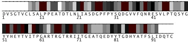
Fig. 1. Residues 1-96 in 1ay7A colored by their relative importance. (See Appendix, Fig.6, for the coloring scheme.)
