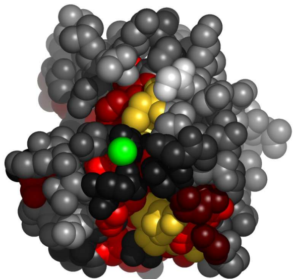
Fig. 6. Residues in 1b08A, at the interface with calcium ion, colored by their relative importance. The ligand (calcium ion) is colored green. Atoms further than 30Å away from the geometric center of the ligand, as well as on the line of sight to the ligand were removed. (See Appendix for the coloring scheme for the protein chain 1b08A.)
