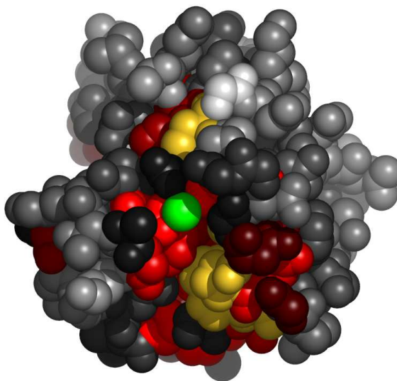
Fig. 4. Residues in 1b08A, at the interface with calcium ion, colored by their relative importance. The ligand (calcium ion) is colored green. Atoms further than 30 Å away from the geometric center of the ligand, as well as on the line of sight to the ligand were removed. (See Appendix for the coloring scheme for the protein chain 1b08A.)
