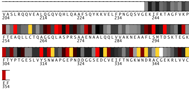
Fig. 1. Residues 204-355 in 1b08A colored by their relative importance. (See Appendix, Fig.10, for the coloring scheme.)
