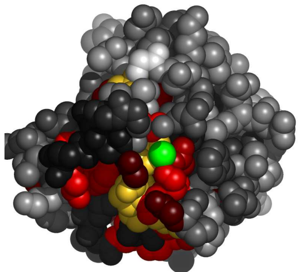
Fig. 7. Residues in 1b08A, at the interface with calcium ion, colored by their relative importance. The ligand (calcium ion) is colored green. Atoms further than 30Å away from the geometric center of the ligand, as well as on the line of sight to the ligand were removed. (See Appendix for the coloring scheme for the protein chain 1b08A.)
