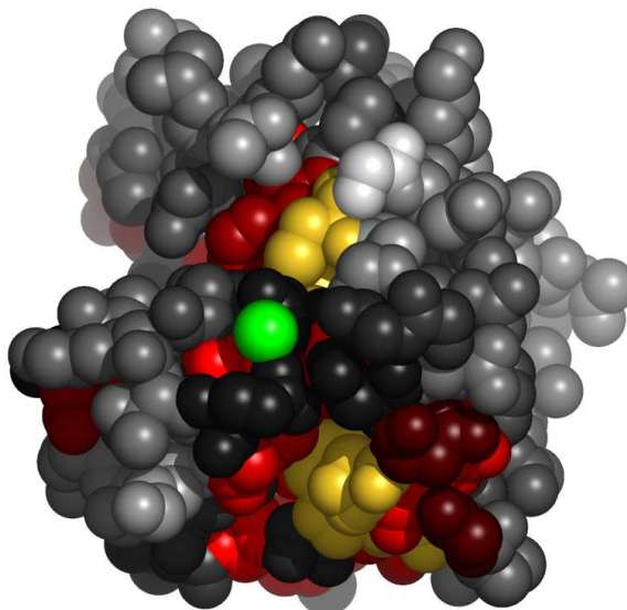
Fig. 8. Residues in 1b08A, at the interface with calcium ion, colored by their relative importance. The ligand (calcium ion) is colored green. Atoms further than 30Å away from the geometric center of the ligand, as well as on the line of sight to the ligand were removed. (See Appendix for the coloring scheme for the protein chain 1b08A.)
