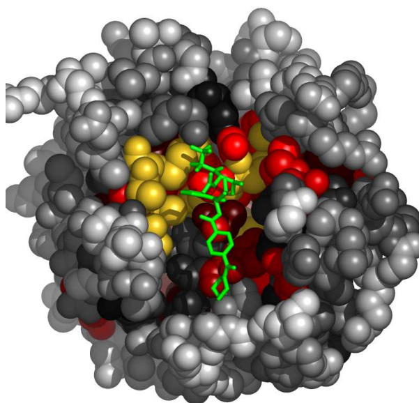
Fig. 9. Residues in 1b0fA, at the interface with SEI, colored by their relative importance. The ligand (SEI) is colored green. Atoms further than 30Å away from the geometric center of the ligand, as well as on the line of sight to the ligand were removed. (See Appendix for the coloring scheme for the protein chain 1b0fA.)
