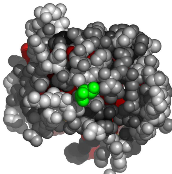
Fig. 8. Residues in 1b0fA, at the interface with alpha-l-fucose, colored by their relative importance. The ligand (alpha-l-fucose) is colored green. Atoms further than 30Å away from the geometric center of the ligand, as well as on the line of sight to the ligand were removed. (See Appendix for the coloring scheme for the protein chain 1b0fA.)
