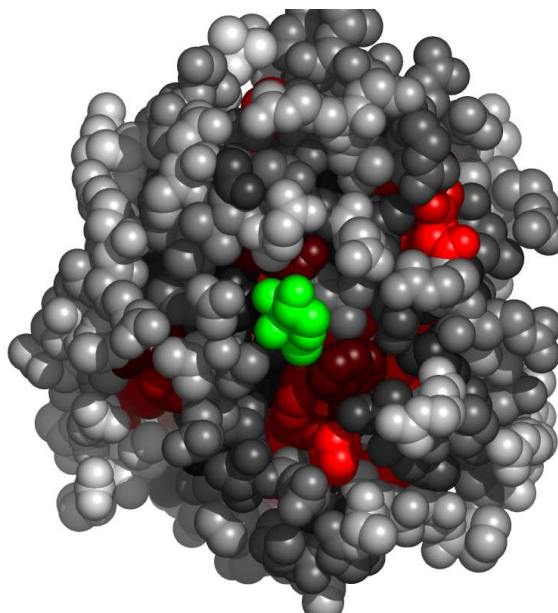
Fig. 6. Residues in 1b0fA, at the interface with alpha-l-fucose, colored by their relative importance. The ligand (alpha-l-fucose) is colored green. Atoms further than 30Å away from the geometric center of the ligand, as well as on the line of sight to the ligand were removed. (See Appendix for the coloring scheme for the protein chain 1b0fA.)
