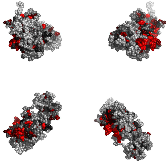
Fig. 3. Residues in 1b3oB, colored by their relative importance. Clockwise: front, back, top and bottom views.
