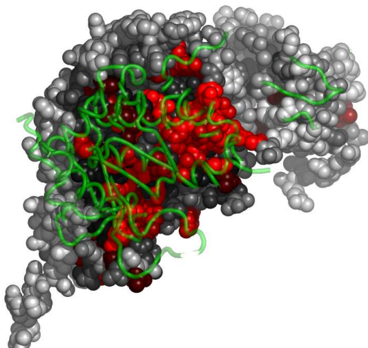
Fig. 8. Residues in 1b3oB, at the interface with 1b3oB3, colored by their relative importance. 1b3oB3 is shown in backbone representation (See Appendix for the coloring scheme for the protein chain 1b3oB.)
