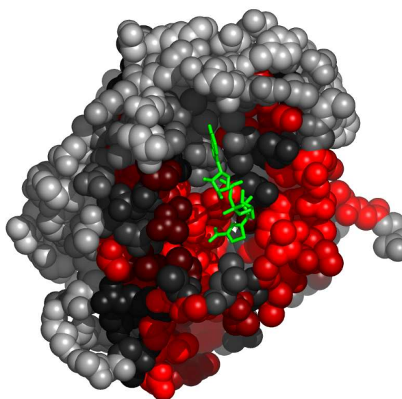
Fig. 9. Residues in 1b3oB, at the interface with SAE, colored by their relative importance. The ligand (SAE) is colored green. Atoms further than 30Å away from the geometric center of the ligand, as well as on the line of sight to the ligand were removed. (See Appendix for the coloring scheme for the protein chain 1b3oB.)
