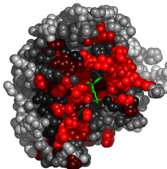
Fig. 6. Residues in 1b3oB, at the interface with CPR, colored by their relative importance. The ligand (CPR) is colored green. Atoms further than 30Å away from the geometric center of the ligand, as well as on the line of sight to the ligand were removed. (See Appendix for the coloring scheme for the protein chain 1b3oB.)
