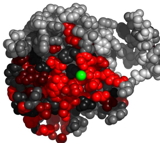
Fig. 5. Residues in 1b3oB, at the interface with unknown atom or ion, colored by their relative importance. The ligand (unknown atom or ion) is colored green. Atoms further than 30Å away from the geometric center of the ligand, as well as on the line of sight to the ligand were removed. (See Appendix for the coloring scheme for the protein chain 1b3oB.)
