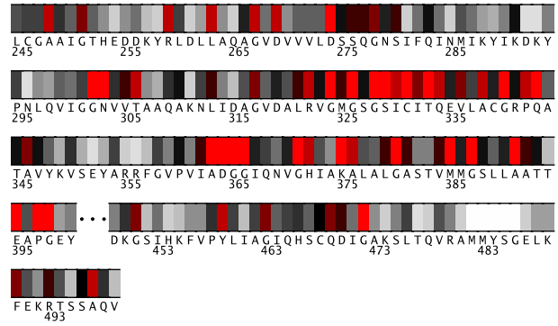
Fig. 2. Residues 245-499 in 1b3oB colored by their relative importance. (See Appendix, Fig.11, for the coloring scheme.)
