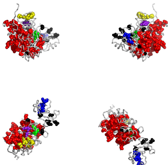
Fig. 4. Residues in 1b3oB, colored according to the cluster they belong to: red, followed by blue and yellow are the largest clusters (see Appendix for the coloring scheme). Clockwise: front, back, top and bottom views. The corresponding Pymol script is attached.
