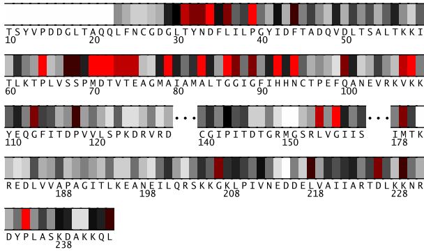
Fig. 1. Residues 10-244 in 1b3oB colored by their relative importance. (See Appendix, Fig.11, for the coloring scheme.)
