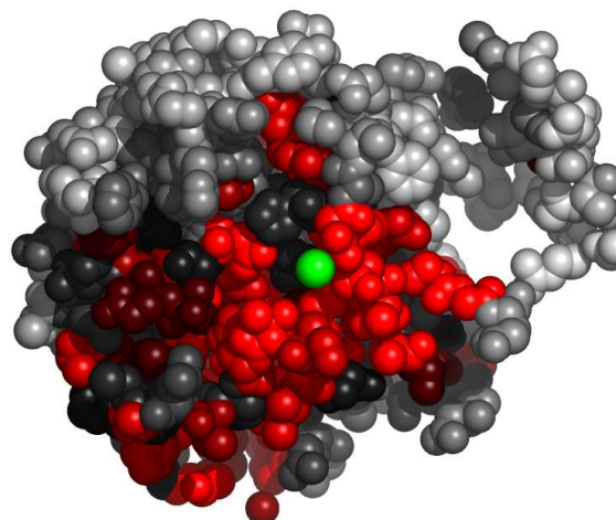
Fig. 7. Residues in 1b3oB, at the interface with unknown atom or ion, colored by their relative importance. The ligand (unknown atom or ion) is colored green. Atoms further than 30Å away from the geometric center of the ligand, as well as on the line of sight to the ligand were removed. (See Appendix for the coloring scheme for the protein chain 1b3oB.)
