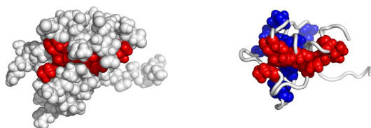
Fig. 5. A possible active surface on the chain 1b50A. The larger cluster it belongs to is shown in blue.
