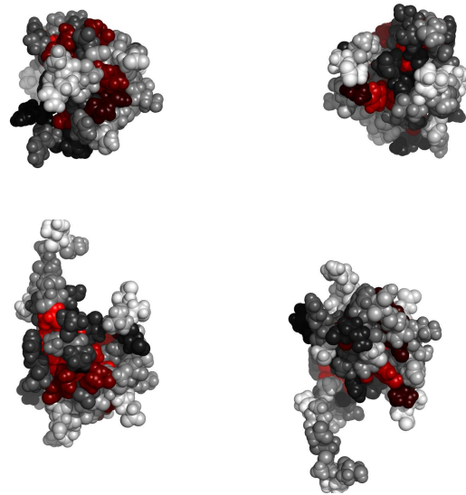
Fig. 2. Residues in 1b50A, colored by their relative importance. Clockwise: front, back, top and bottom views.
