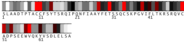
Fig. 1. Residues 1-69 in 1b50A colored by their relative importance. (See Appendix, Fig.6, for the coloring scheme.)
