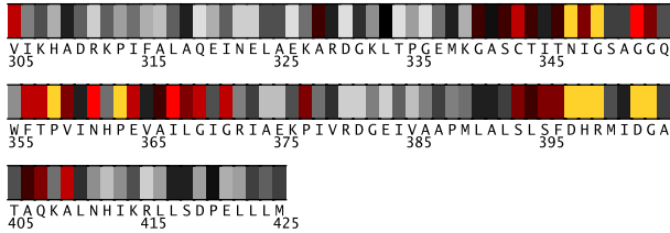
Fig. 2. Residues 305-425 in 1b5sA colored by their relative importance. (See Appendix, Fig.9, for the coloring scheme.)
