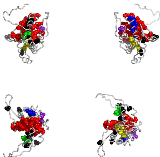
Fig. 4. Residues in 1b5sA, colored according to the cluster they belong to: red, followed by blue and yellow are the largest clusters (see Appendix for the coloring scheme). Clockwise: front, back, top and bottom views. The corresponding Pymol script is attached.
