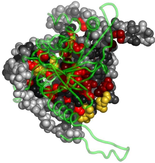
Fig. 6. Residues in 1b5sA, at the interface with 1b5sA2, colored by their relative importance. 1b5sA2 is shown in backbone representation (See Appendix for the coloring scheme for the protein chain 1b5sA.)
