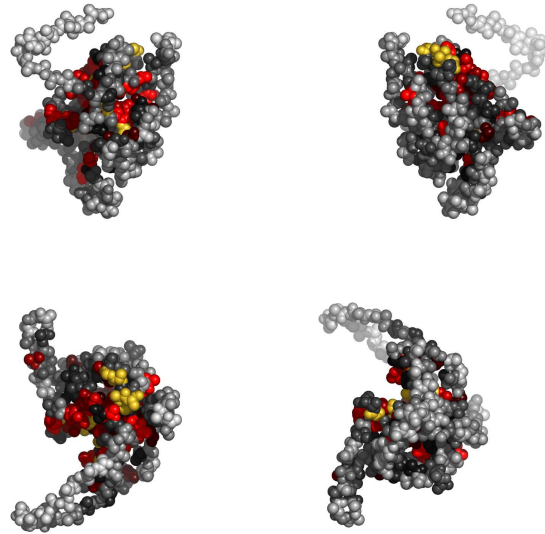
Fig. 3. Residues in 1b5sA, colored by their relative importance. Clockwise: front, back, top and bottom views.
