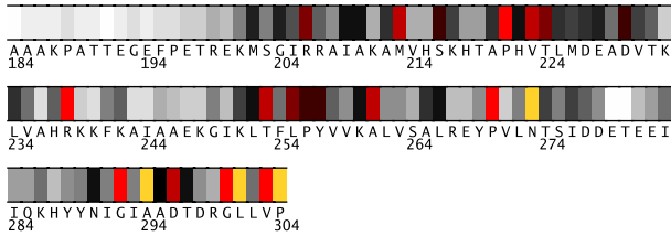
Fig. 1. Residues 184-304 in 1b5sA colored by their relative importance. (See Appendix, Fig.9, for the coloring scheme.)
