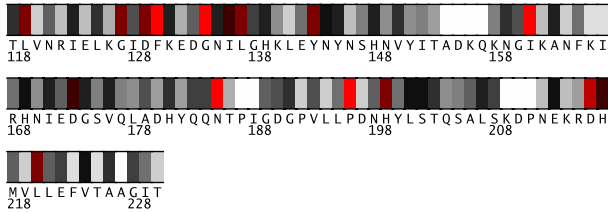
Fig. 2. Residues 118-230 in 1b9cA colored by their relative importance. (See Appendix, Fig.9, for the coloring scheme.)
