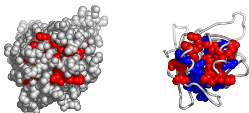
Fig. 7. A possible active surface on the chain 1b9cA. The larger cluster it belongs to is shown in blue.
