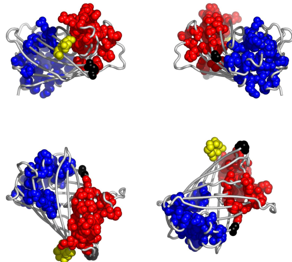
Fig. 4. Residues in 1b9cA, colored according to the cluster they belong to: red, followed by blue and yellow are the largest clusters (see Appendix for the coloring scheme). Clockwise: front, back, top and bottom views. The corresponding Pymol script is attached.
