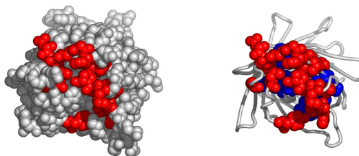
Fig. 8. Another possible active surface on the chain 1b9cA. The larger cluster it belongs to is shown in blue.
