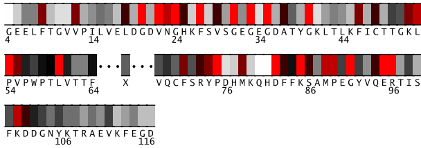
Fig. 1. Residues 4-117 in 1b9cA colored by their relative importance. (See Appendix, Fig.9, for the coloring scheme.)
