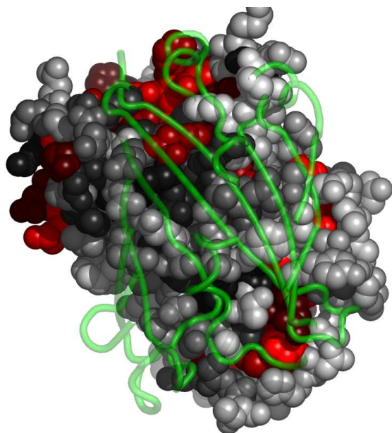
Fig. 6. Residues in 1b9cA, at the interface with 1b9cD, colored by their relative importance. 1b9cD is shown in backbone representation (See Appendix for the coloring scheme for the protein chain 1b9cA.)
