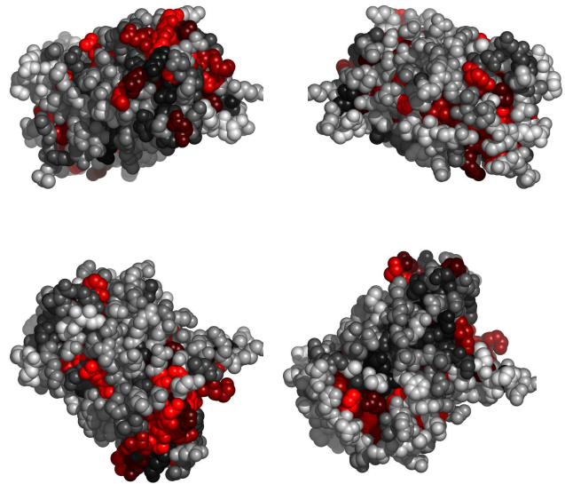
Fig. 3. Residues in 1b9cA, colored by their relative importance. Clockwise: front, back, top and bottom views.
