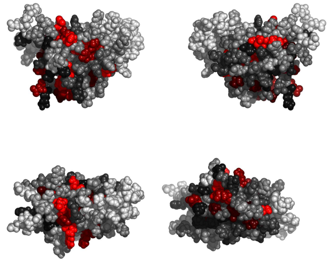
Fig. 1. Residues 1-133 in 1bbnA colored by their relative importance. (See Appendix, Fig.6, for the coloring scheme.)
