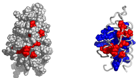
Fig. 4. A possible active surface on the chain 1bbnA. The larger cluster it belongs to is shown in blue.
