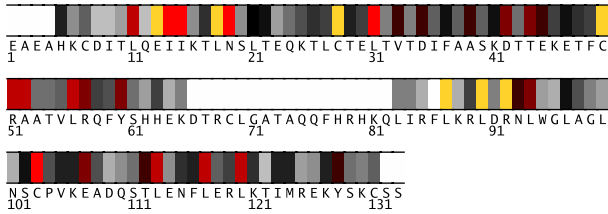
Fig. 1. Residues 1-133 in 1bbnA colored by their relative importance. (See Appendix, Fig.6, for the coloring scheme.)
