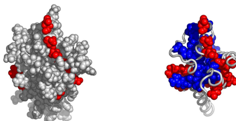
Fig. 5. Another possible active surface on the chain 1bbnA. The larger cluster it belongs to is shown in blue.
