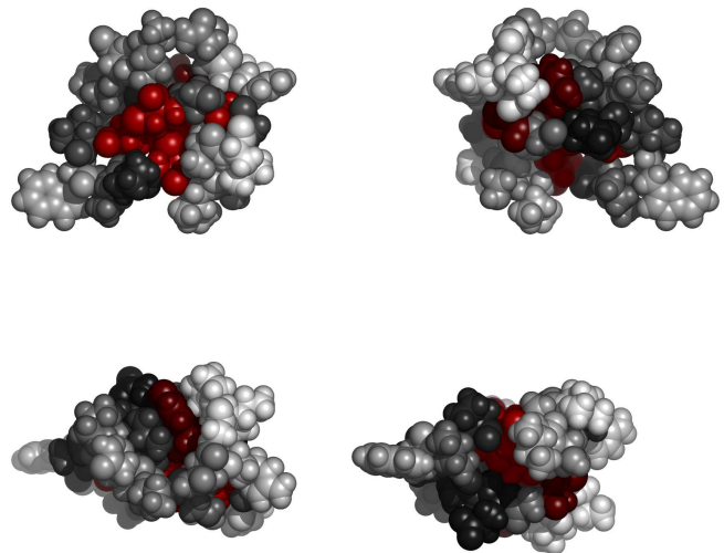
Fig. 1. Residues 1-30 in 1bh4A colored by their relative importance. (See Appendix, Fig.5, for the coloring scheme.)
