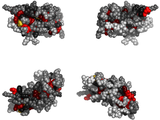
Fig. 1. Residues 1-98 in 1bmgA colored by their relative importance. (See Appendix, Fig.6, for the coloring scheme.)
