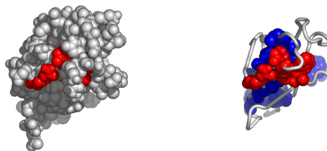
Fig. 5. Another possible active surface on the chain 1bmgA. The larger cluster it belongs to is shown in blue.
