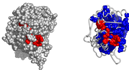
Fig. 8. Another possible active surface on the chain 1bo7A. The larger cluster it belongs to is shown in blue.
