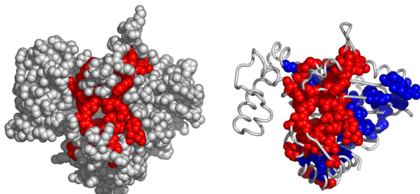
Fig. 7. A possible active surface on the chain Ibo7A. The larger cluster it belongs to is shown in blue.
