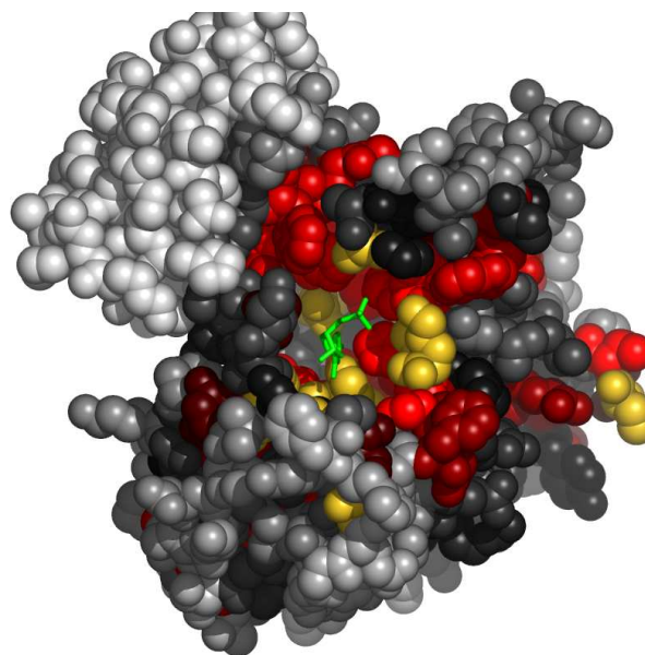
Fig. 5. Residues in 1bo7A, at the interface with U, colored by their relative importance. The ligand (U) is colored green. Atoms further than 30Å away from the geometric center of the ligand, as well as on the line of sight to the ligand were removed. (See Appendix for the coloring scheme for the protein chain 1bo7A.)
