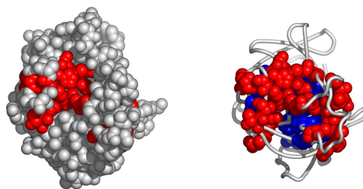
Fig. 6. A possible active surface on the chain IboqA. The larger cluster it belongs to is shown in blue.
