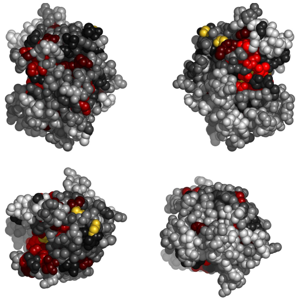
Fig. 2. Residues in IboqA, colored by their relative importance. Clockwise: front, back, top and bottom views.
