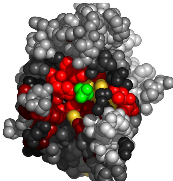
Fig. 5. Residues in IboqA, at the interface with sulfate ion, colored by their relative importance. The ligand (sulfate ion) is colored green. Atoms further than 30Å away from the geometric center of the ligand, as well as on the line of sight to the ligand were removed. (See Appendix for the coloring scheme for the protein chain IboqA.)
