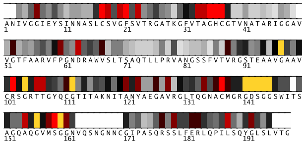
Fig. 1. Residues 1-198 in IboqA colored by their relative importance. (See Appendix, Fig.7, for the coloring scheme.)
