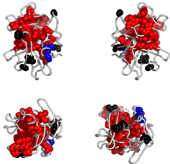
Fig. 2. Residues in IboqA, colored by their relative importance. Clockwise: front, back, top and bottom views.
