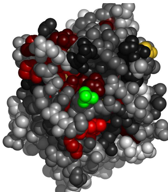
Fig. 4. Residues in 1boqA, at the interface with sulfate ion, colored by their relative importance. The ligand (sulfate ion) is colored green. Atoms further than 30Å away from the geometric center of the ligand, as well as on the line of sight to the ligand were removed. (See Appendix for the coloring scheme for the protein chain 1boqA.)
