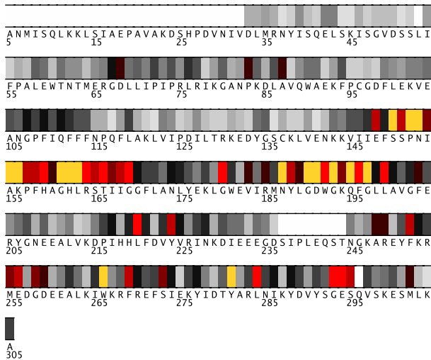
Fig. 1. Residues 5-305 in 1bs2A colored by their relative importance. (See Appendix, Fig.6, for the coloring scheme.)
