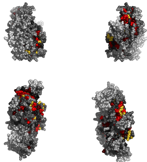
Fig. 3. Residues in 1bs2A, colored by their relative importance. Clockwise: front, back, top and bottom views.
