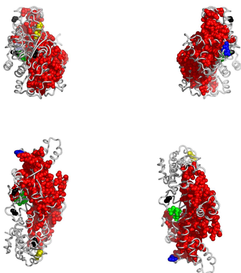
Fig. 4. Residues in 1bs2A, colored according to the cluster they belong to: red, followed by blue and yellow are the largest clusters (see Appendix for the coloring scheme). Clockwise: front, back, top and bottom views. The corresponding Pymol script is attached.
