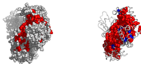
Fig. 5. A possible active surface on the chain 1bs2A. The larger cluster it belongs to is shown in blue.
