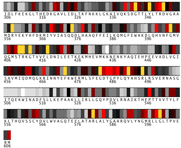
Fig. 2. Residues 306-607 in 1bs2A colored by their relative importance. (See Appendix, Fig.6, for the coloring scheme.)
