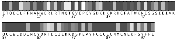
Fig. 1. Residues 7-100 in 1bteB colored by their relative importance. (See Appendix, Fig.4, for the coloring scheme.)
