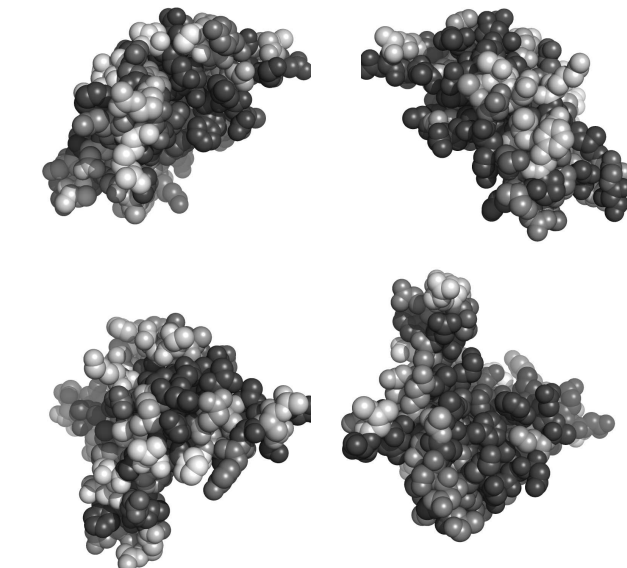
Fig. 2. Residues in 1bteB, colored by their relative importance. Clockwise: front, back, top and bottom views.
