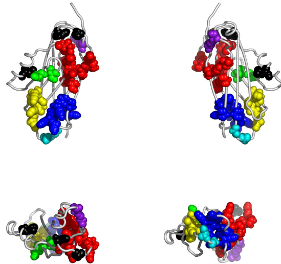
Fig. 2. Residues in 1bv8A, colored by their relative importance. Clockwise: front, back, top and bottom views.
