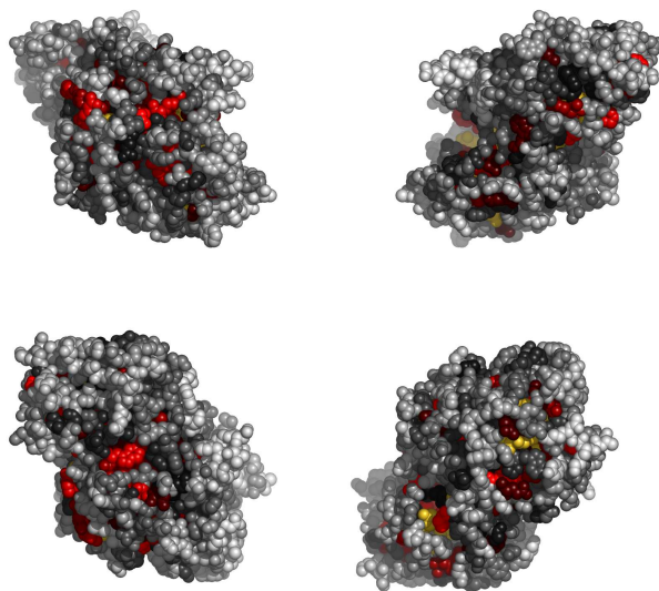
Fig. 3. Residues in 1bnvP, colored by their relative importance. Clockwise: front, back, top and bottom views.
