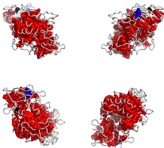
Fig. 4. Residues in 1bvnP, colored according to the cluster they belong to: red, followed by blue and yellow are the largest clusters (see Appendix for the coloring scheme). Clockwise: front, back, top and bottom views. The corresponding Pymol script is attached.
