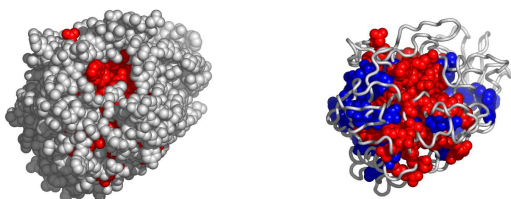
Fig. 9. Another possible active surface on the chain 1bvnP. The larger cluster it belongs to is shown in blue.
