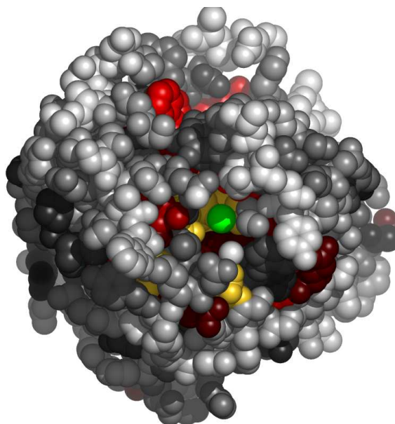
Fig. 5. Residues in 1bvnP, at the interface with calcium ion, colored by their relative importance. The ligand (calcium ion) is colored green. Atoms further than 30Å away from the geometric center of the ligand, as well as on the line of sight to the ligand were removed. (See Appendix for the coloring scheme for the protein chain 1bvnP.)
