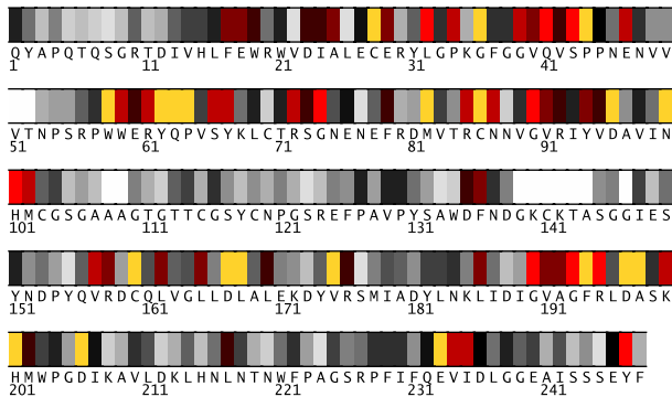
Fig. 1. Residues 1-248 in 1bnvP colored by their relative importance. (See Appendix, Fig.10, for the coloring scheme.)
