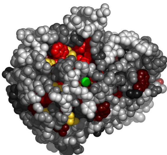
Fig. 7. Residues in 1bvnP, at the interface with chloride ion, colored by their relative importance. The ligand (chloride ion) is colored green. Atoms further than 30Å away from the geometric center of the ligand, as well as on the line of sight to the ligand were removed. (See Appendix for the coloring scheme for the protein chain 1bvnP.)
