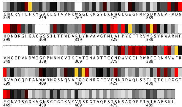
Fig. 2. Residues 249-496 in 1bnvP colored by their relative importance. (See Appendix, Fig.10, for the coloring scheme.)
