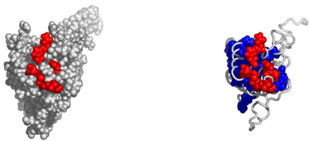
Fig. 6. Another possible active surface on the chain 1bx1A. The larger cluster it belongs to is shown in blue.
