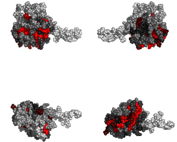
Fig. 1. Residues -3-217 in 1bx1A colored by their relative importance. (See Appendix, Fig.7, for the coloring scheme.)
