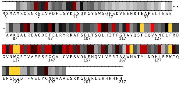
Fig. 1. Residues -3-217 in 1bx1A colored by their relative importance. (See Appendix, Fig.7, for the coloring scheme.)
