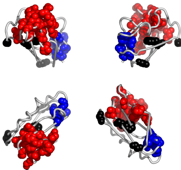
Fig. 3. Residues in IbyoA, colored according to the cluster they belong to: red, followed by blue and yellow are the largest clusters (see Appendix for the coloring scheme). Clockwise: front, back, top and bottom views. The corresponding Pymol script is attached.
