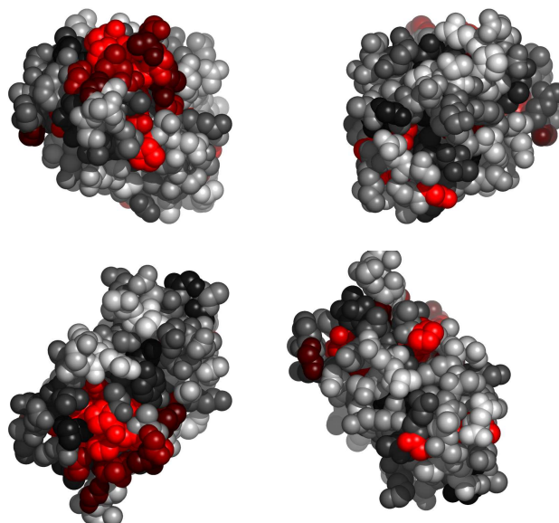
Fig. 2. Residues in IbyoA, colored by their relative importance. Clockwise: front, back, top and bottom views.
