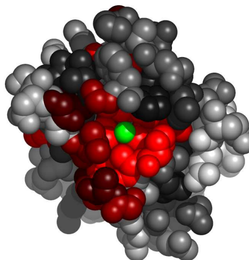
Fig. 4. Residues in 1byoA, at the interface with copper (ii) ion, colored by their relative importance. The ligand (copper (ii) ion) is colored green. Atoms further than 30Å away from the geometric center of the ligand, as well as on the line of sight to the ligand were removed. (See Appendix for the coloring scheme for the protein chain 1byoA.)
