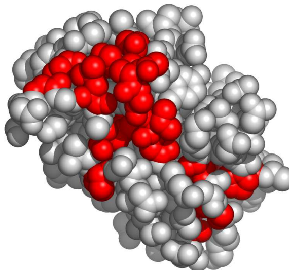
Fig. 5. A possible active surface on the chain 1byoA.
