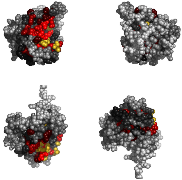
Fig. 3. Residues in 1byqA, colored by their relative importance. Clockwise: front, back, top and bottom views.
