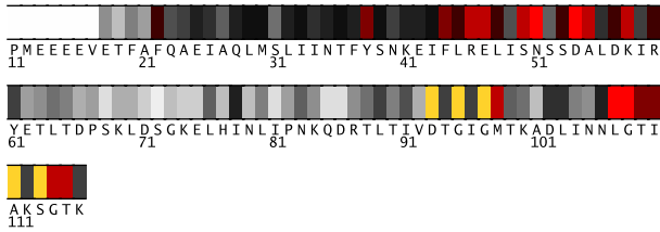
Fig. 1. Residues 11-116 in 1byqA colored by their relative importance. (See Appendix, Fig.7, for the coloring scheme.)
