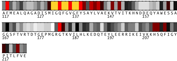
Fig. 2. Residues 117-223 in 1byqA colored by their relative importance. (See Appendix, Fig.7, for the coloring scheme.)
