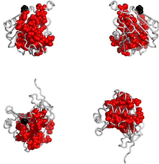
Fig. 4. Residues in 1byqA, colored according to the cluster they belong to: red, followed by blue and yellow are the largest clusters (see Appendix for the coloring scheme). Clockwise: front, back, top and bottom views. The corresponding Pymol script is attached.
