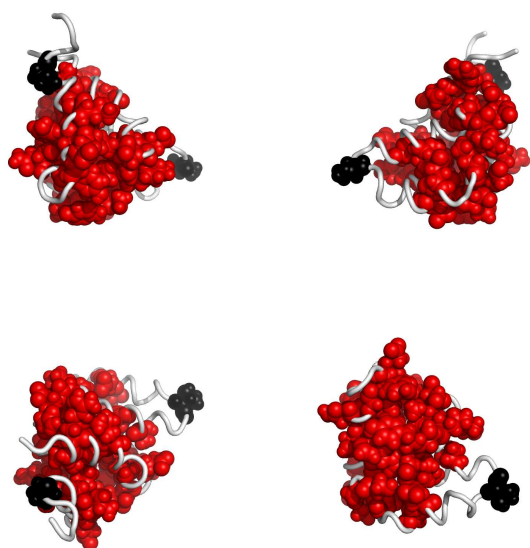
Fig. 3. Residues in 1c15A, colored according to the cluster they belong to: red, followed by blue and yellow are the largest clusters (see Appendix for the coloring scheme). Clockwise: front, back, top and bottom views. The corresponding Pymol script is attached.
