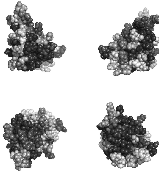
Fig. 2. Residues in 1c15A, colored by their relative importance. Clockwise: front, back, top and bottom views.
