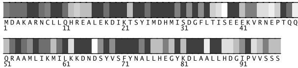
Fig. 1. Residues 1-97 in 1c15A colored by their relative importance. (See Appendix, Fig.4, for the coloring scheme.)
