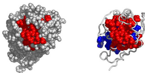
Fig. 9. Another possible active surface on the chain 1cb0A. The larger cluster it belongs to is shown in blue.
