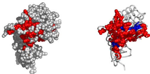
Fig. 6. A possible active surface on the chain IckiA. The larger cluster it belongs to is shown in blue.
