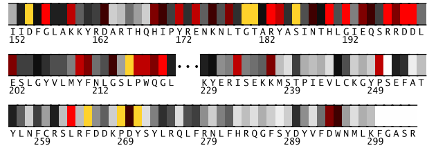
Fig. 2. Residues 152-304 in IckiA colored by their relative importance. (See Appendix, Fig.7, for the coloring scheme.)
