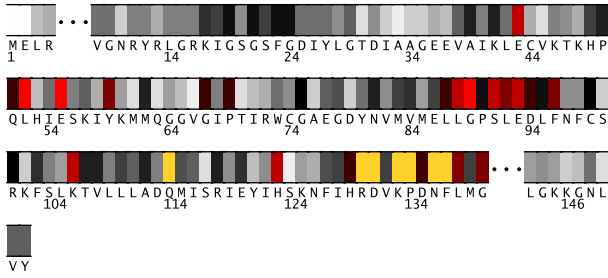
Fig. 1. Residues 1-151 in IckiA colored by their relative importance. (See Appendix, Fig.7, for the coloring scheme.)
