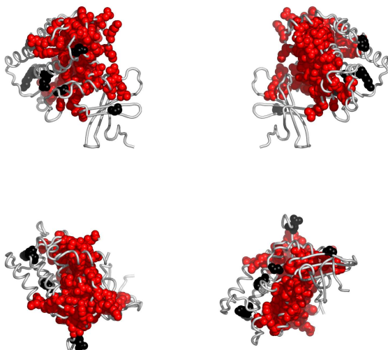
Fig. 4. Residues in 1ckiA, colored according to the cluster they belong to: red, followed by blue and yellow are the largest clusters (see Appendix for the coloring scheme). Clockwise: front, back, top and bottom views. The corresponding Pymol script is attached.
