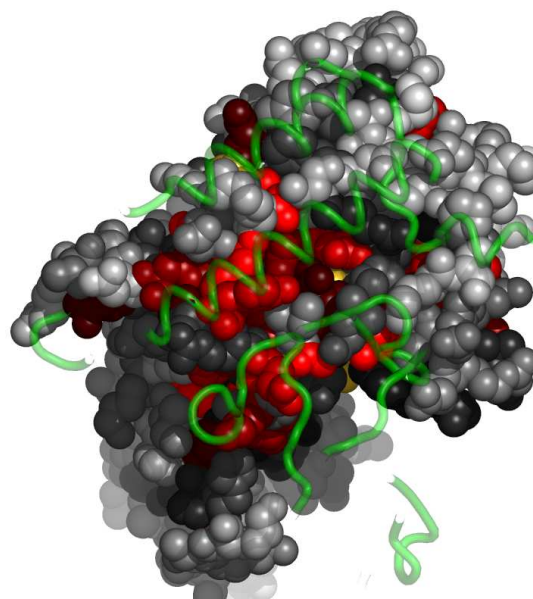
Fig. 5. Residues in 1ckiA, at the interface with 1ckiB, colored by their relative importance. 1ckiB is shown in backbone representation (See Appendix for the coloring scheme for the protein chain 1ckiA.)
