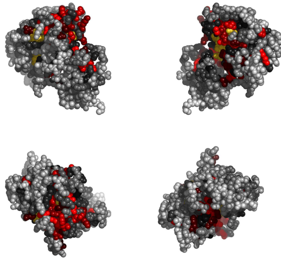
Fig. 3. Residues in IckiA, colored by their relative importance. Clockwise: front, back, top and bottom views.
