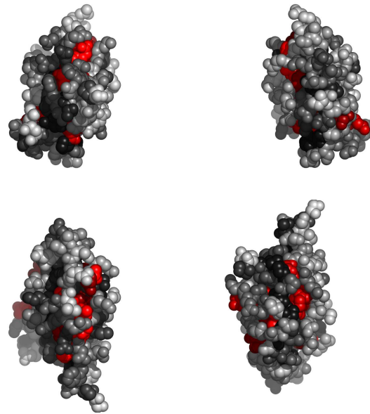
Fig. 2. Residues in 1csgA, colored by their relative importance. Clockwise: front, back, top and bottom views.
