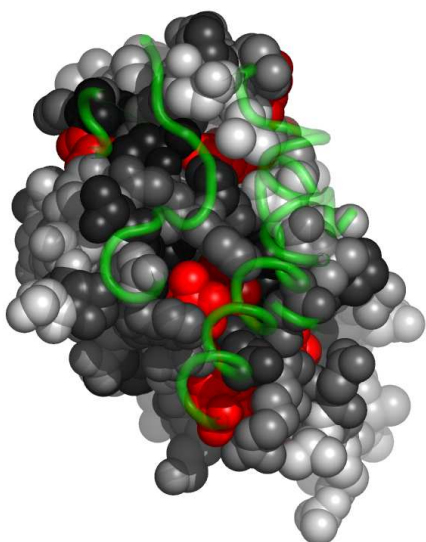
Fig. 4. Residues in 1csgA, at the interface with 1csgB, colored by their relative importance. 1csgB is shown in backbone representation (See Appendix for the coloring scheme for the protein chain 1csgA.)
