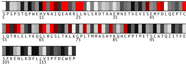
Fig. 1. Residues 5-124 in 1csgA colored by their relative importance. (See Appendix, Fig.7, for the coloring scheme.)
