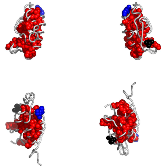
Fig. 3. Residues in 1csgA, colored according to the cluster they belong to: red, followed by blue and yellow are the largest clusters (see Appendix for the coloring scheme). Clockwise: front, back, top and bottom views. The corresponding Pymol script is attached.
