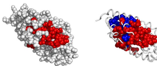
Fig. 6. A possible active surface on the chain 1db1A. The larger cluster it belongs to is shown in blue.
