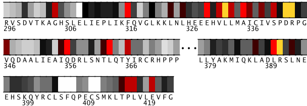
Fig. 2. Residues 296-423 in Idb1A colored by their relative importance. (See Appendix, Fig.7, for the coloring scheme.)
