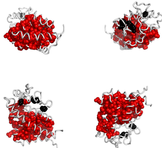
Fig. 4. Residues in Idb1A, colored according to the cluster they belong to: red, followed by blue and yellow are the largest clusters (see Appendix for the coloring scheme). Clockwise: front, back, top and bottom views. The corresponding Pymol script is attached.
