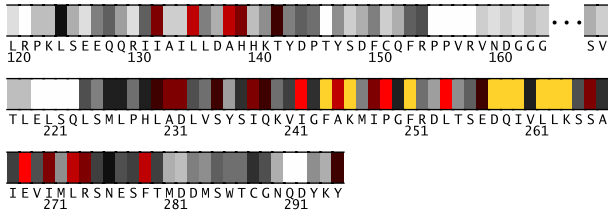
Fig. 1. Residues 120-295 in Idb1A colored by their relative importance. (See Appendix, Fig.7, for the coloring scheme.)
