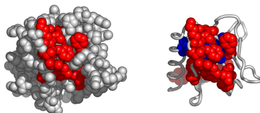
Fig. 5. A possible active surface on the chain 1ddvA. The larger cluster it belongs to is shown in blue.
