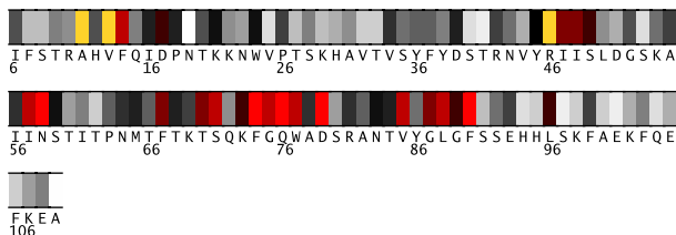
Fig. 1. Residues 6-109 in 1ddvA colored by their relative importance. (See Appendix, Fig.6, for the coloring scheme.)
