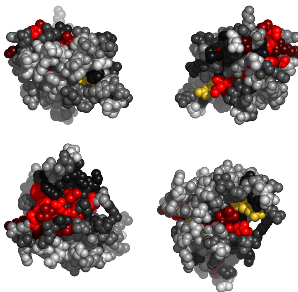
Fig. 2. Residues in 1ddvA, colored by their relative importance. Clockwise: front, back, top and bottom views.
