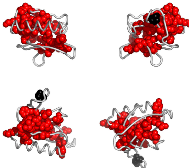
Fig. 3. Residues in 1ddvA, colored according to the cluster they belong to: red, followed by blue and yellow are the largest clusters (see Appendix for the coloring scheme). Clockwise: front, back, top and bottom views. The corresponding Pymol script is attached.
