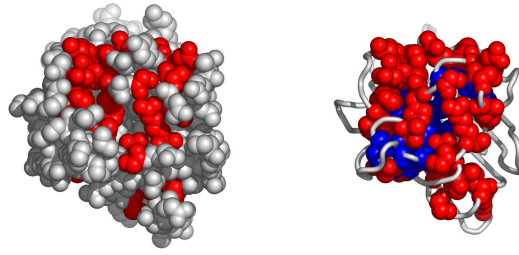
Fig. 7. A possible active surface on the chain 1do5A. The larger cluster it belongs to is shown in blue.
