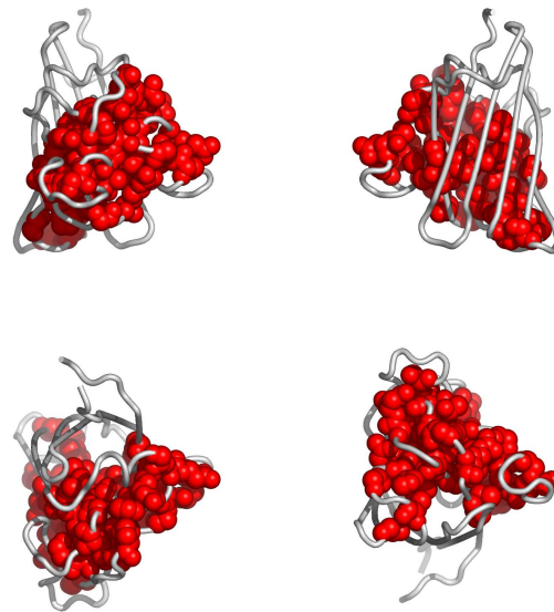
Fig. 3. Residues in 1do5A, colored according to the cluster they belong to: red, followed by blue and yellow are the largest clusters (see Appendix for the coloring scheme). Clockwise: front, back, top and bottom views. The corresponding Pymol script is attached.
