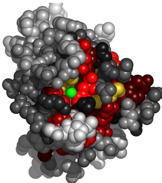
Fig. 5. Residues in 1do5A, at the interface with zinc ion, colored by their relative importance. The ligand (zinc ion) is colored green. Atoms further than 30Å away from the geometric center of the ligand, as well as on the line of sight to the ligand were removed. (See Appendix for the coloring scheme for the protein chain 1do5A.)
