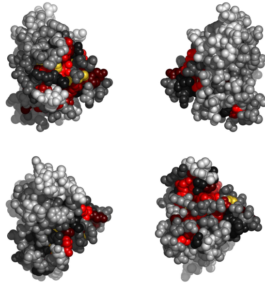
Fig. 2. Residues in 1do5A, colored by their relative importance. Clockwise: front, back, top and bottom views.
