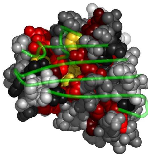
Fig. 4. Residues in 1do5A, at the interface with 1do5D, colored by their relative importance. 1do5D is shown in backbone representation (See Appendix for the coloring scheme for the protein chain 1do5A.)
