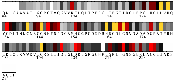
Fig. 1. Residues 84-237 in 1do5A colored by their relative importance. (See Appendix, Fig.8, for the coloring scheme.)
