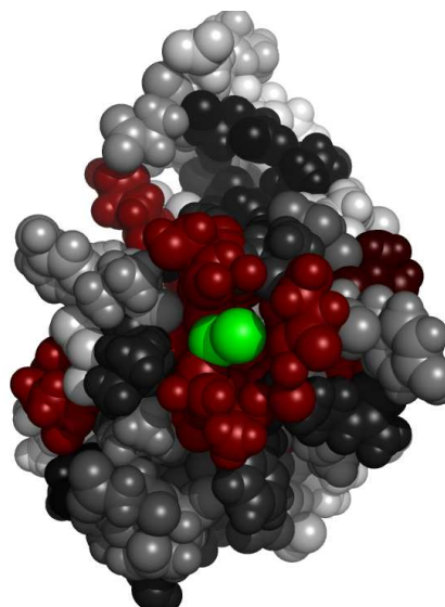
Fig. 4. Residues in 1doxA, at the interface with FES, colored by their relative importance. The ligand (FES) is colored green. Atoms further than 30Å away from the geometric center of the ligand, as well as on the line of sight to the ligand were removed. (See Appendix for the coloring scheme for the protein chain 1doxA.)
