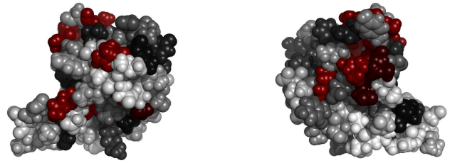
Fig. 1. Residues 1-96 in 1doxA colored by their relative importance. (See Appendix, Fig.6, for the coloring scheme.)
