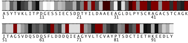
Fig. 1. Residues 1-96 in 1doxA colored by their relative importance. (See Appendix, Fig.6, for the coloring scheme.)
