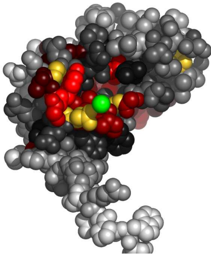
Fig. 6. Residues in 1ducA, at the interface with strontium ion, colored by their relative importance. The ligand (strontium ion) is colored green. Atoms further than 30Å away from the geometric center of the ligand, as well as on the line of sight to the ligand were removed. (See Appendix for the coloring scheme for the protein chain 1ducA.)
