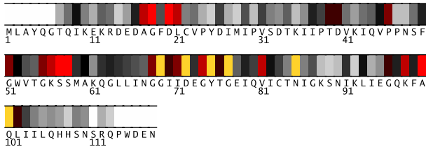
Fig. 1. Residues 1-118 in 1ducA colored by their relative importance. (See Appendix, Fig.8, for the coloring scheme.)
