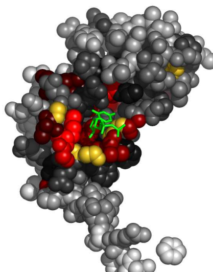
Fig. 7. Residues in 1ducA, at the interface with DUD, colored by their relative importance. The ligand (DUD) is colored green. Atoms further than 30Å away from the geometric center of the ligand, as well as on the line of sight to the ligand were removed. (See Appendix for the coloring scheme for the protein chain 1ducA.)
