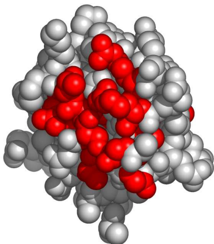
Fig. 6. A possible active surface on the chain 1dulA.
