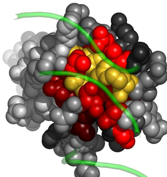
Fig. 4. Residues in 1dulA, at the interface with DNA (1dulB), colored by their relative importance. DNA is colored green. (See Appendix for the coloring scheme for the protein chain 1dulA.)
