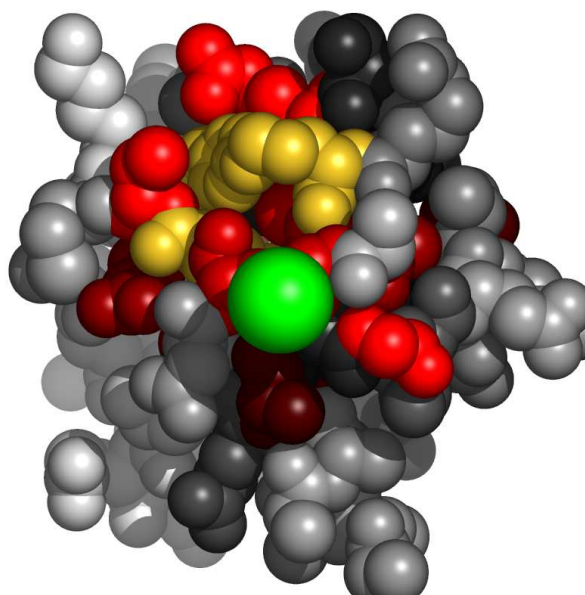
Fig. 5. Residues in 1dulA, at the interface with potassium ion, colored by their relative importance. The ligand (potassium ion) is colored green. Atoms further than 30Å away from the geometric center of the ligand, as well as on the line of sight to the ligand were removed. (See Appendix for the coloring scheme for the protein chain 1dulA.)
