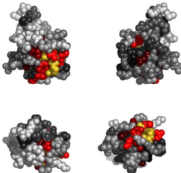
Fig. 2. Residues in 1dulA, colored by their relative importance. Clockwise: front, back, top and bottom views.
