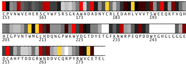
Fig. 1. Residues 153-280 in 1dv8A colored by their relative importance. (See Appendix, Fig.8, for the coloring scheme.)
