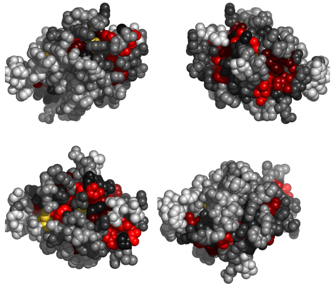
Fig. 2. Residues in 1dv8A, colored by their relative importance. Clockwise: front, back, top and bottom views.
