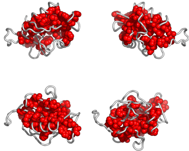
Fig. 3. Residues in 1dv8A, colored according to the cluster they belong to: red, followed by blue and yellow are the largest clusters (see Appendix for the coloring scheme). Clockwise: front, back, top and bottom views. The corresponding Pymol script is attached.
