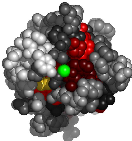
Fig. 4. Residues in 1dv8A, at the interface with calcium ion, colored by their relative importance. The ligand (calcium ion) is colored green. Atoms further than 30 Å away from the geometric center of the ligand, as well as on the line of sight to the ligand were removed. (See Appendix for the coloring scheme for the protein chain 1dv8A.)
