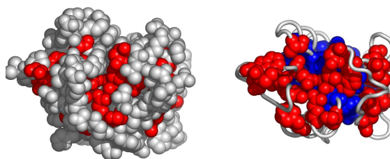
Fig. 7. A possible active surface on the chain 1dv8A. The larger cluster it belongs to is shown in blue.
