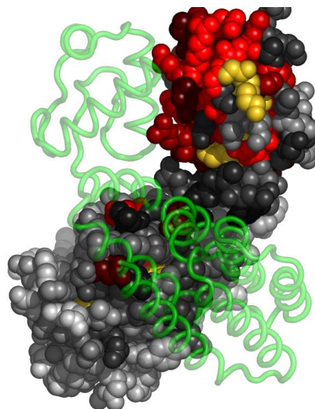
Fig. 6. Residues in 1e2xA, at the interface with 1e2xA1, colored by their relative importance. 1e2xA1 is shown in backbone representation (See Appendix for the coloring scheme for the protein chain 1e2xA.)
