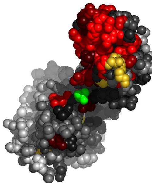
Fig. 5. Residues in 1e2xA, at the interface with sulfate ion, colored by their relative importance. The ligand (sulfate ion) is colored green. Atoms further than 30 Å away from the geometric center of the ligand, as well as on the line of sight to the ligand were removed. (See Appendix for the coloring scheme for the protein chain 1e2xA.)
