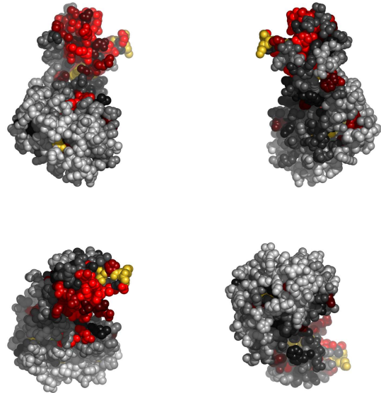
Fig. 3. Residues in 1e2xA, colored by their relative importance. Clockwise: front, back, top and bottom views.
