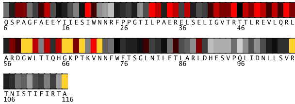
Fig. 1. Residues 6-116 in 1e2xA colored by their relative importance. (See Appendix, Fig.9, for the coloring scheme.)
