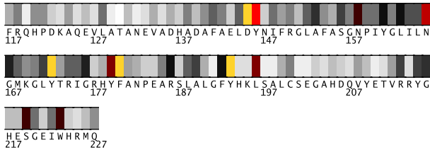
Fig. 2. Residues 117-227 in 1e2xA colored by their relative importance. (See Appendix, Fig.9, for the coloring scheme.)
