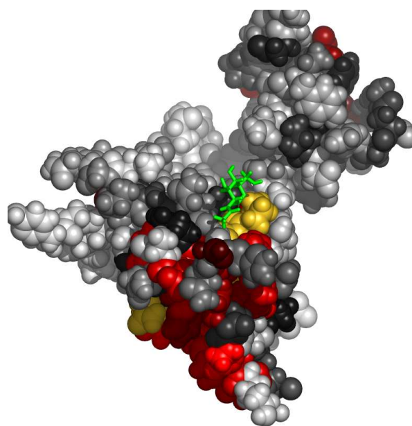
Fig. 4. Residues in 1e88A, at the interface with NAG, colored by their relative importance. The ligand (NAG) is colored green. Atoms further than 30 Å away from the geometric center of the ligand, as well as on the line of sight to the ligand were removed. (See Appendix for the coloring scheme for the protein chain 1e88A.)
