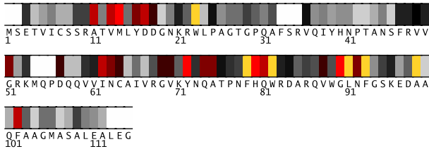
Fig. 1. Residues 1-115 in legxA colored by their relative importance. (See Appendix, Fig.5, for the coloring scheme.)
