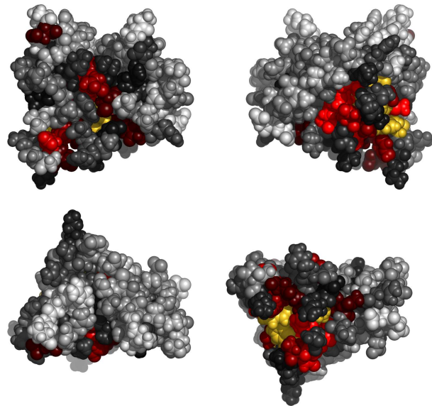
Fig. 2. Residues in legxA, colored by their relative importance. Clockwise: front, back, top and bottom views.
