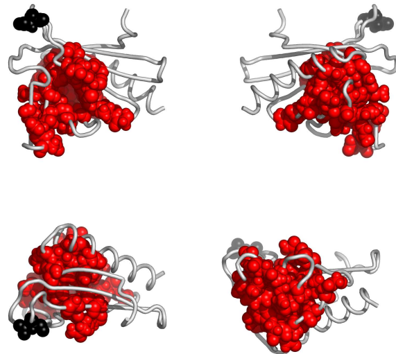
Fig. 2. Residues in legxA, colored by their relative importance. Clockwise: front, back, top and bottom views.
