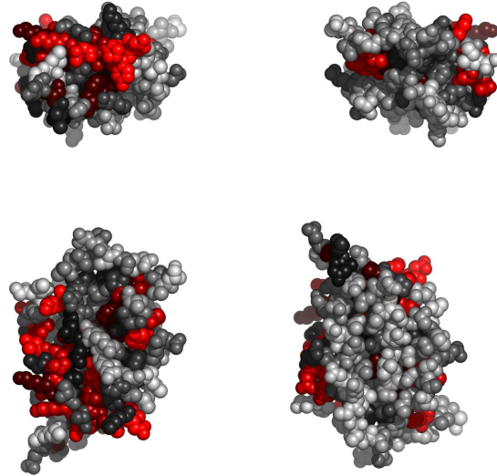
Fig. 2. Residues in IexzB, colored by their relative importance. Clockwise: front, back, top and bottom views.
