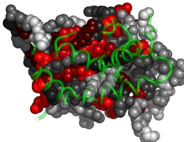
Fig. 4. Residues in 1exzB, at the interface with 1exzC, colored by their relative importance. 1exzC is shown in backbone representation (See Appendix for the coloring scheme for the protein chain 1exzB.)
