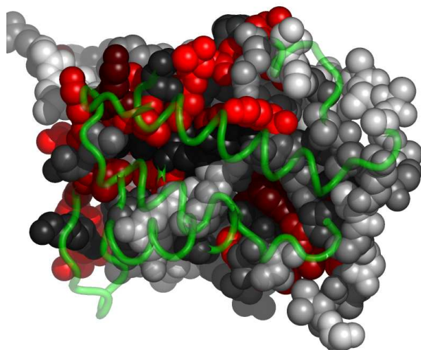
Fig. 5. Residues in 1exzB, at the interface with 1exzA, colored by their relative importance. 1exzA is shown in backbone representation (See Appendix for the coloring scheme for the protein chain 1exzB.)
