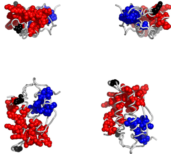
Fig. 3. Residues in IexzB, colored according to the cluster they belong to: red, followed by blue and yellow are the largest clusters (see Appendix for the coloring scheme). Clockwise: front, back, top and bottom views. The corresponding Pymol script is attached.
