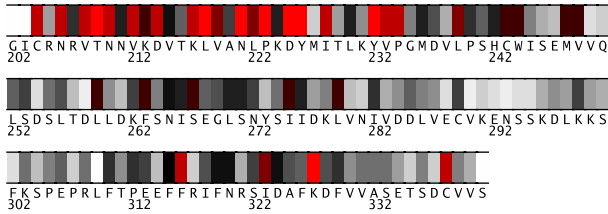
Fig. 1. Residues 202-341 in IexzB colored by their relative importance. (See Appendix, Fig.9, for the coloring scheme.)
