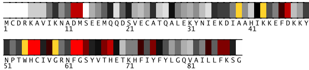
Fig. 1. Residues 1-89 in 1f3cA colored by their relative importance. (See Appendix, Fig.6, for the coloring scheme.)
