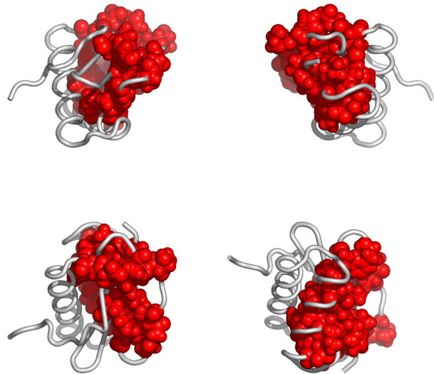
Fig. 3. Residues in 1f3cA, colored according to the cluster they belong to: red, followed by blue and yellow are the largest clusters (see Appendix for the coloring scheme). Clockwise: front, back, top and bottom views. The corresponding Pymol script is attached.
