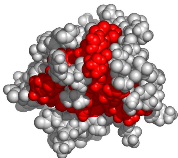
Fig. 5. A possible active surface on the chain 1f3cA.
