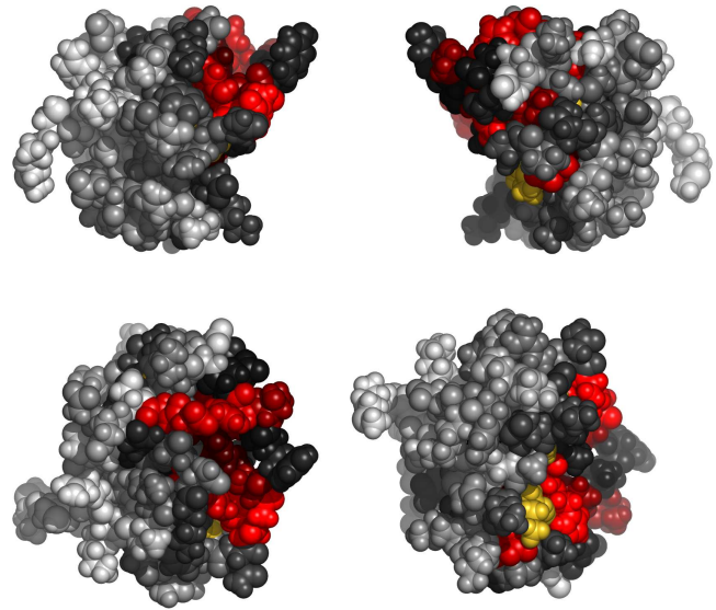
Fig. 2. Residues in 1f3cA, colored by their relative importance. Clockwise: front, back, top and bottom views.
