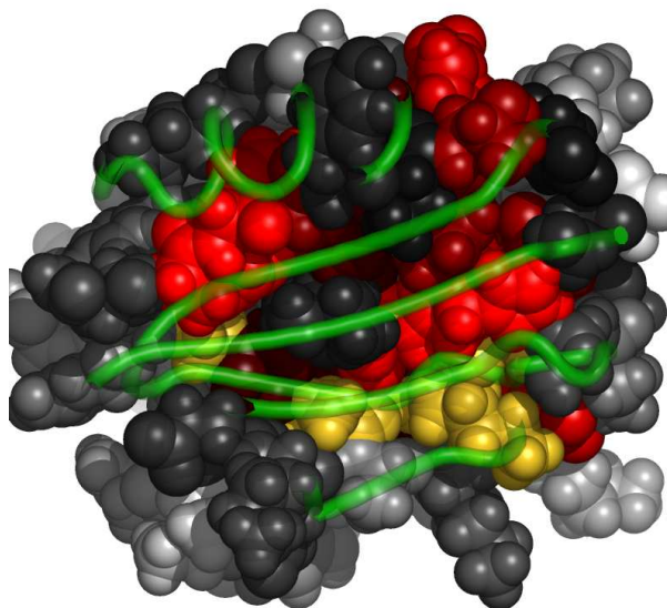
Fig. 4. Residues in 1f3cA, at the interface with 1f3cB, colored by their relative importance. 1f3cB is shown in backbone representation (See Appendix for the coloring scheme for the protein chain 1f3cA.)
