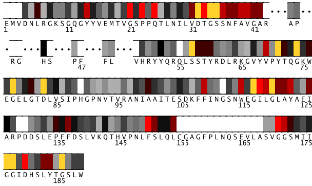
Fig. 1. Residues 1-189 in 1fkNA colored by their relative importance. (See Appendix, Fig.8, for the coloring scheme.) Note that some residues in 1fkNA carry insertion code.
