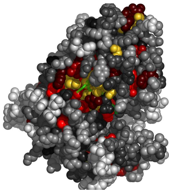
Fig. 5. Residues in 1fknA, at the interface with 1fknC, colored by their relative importance. 1fknC is shown in backbone representation (See Appendix for the coloring scheme for the protein chain 1fknA.)
