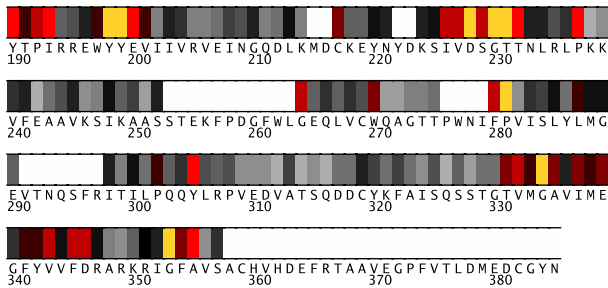
Fig. 2. Residues 190-385 in 1fkNA colored by their relative importance. (See Appendix, Fig.8, for the coloring scheme.) Note that some residues in 1fkNA carry insertion code.
