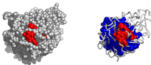
Fig. 6. A possible active surface on the chain 1fknA. The larger cluster it belongs to is shown in blue.
