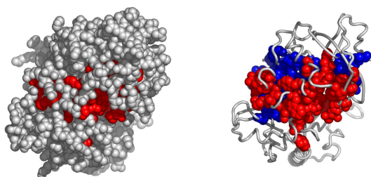
Fig. 7. Another possible active surface on the chain 1fknA. The larger cluster it belongs to is shown in blue.
