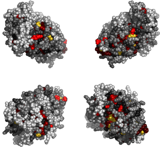
Fig. 3. Residues in 1fkNA, colored by their relative importance. Clockwise: front, back, top and bottom views.
