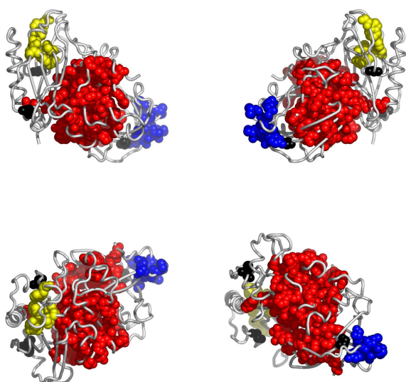
Fig. 4. Residues in 1fknA, colored according to the cluster they belong to: red, followed by blue and yellow are the largest clusters (see Appendix for the coloring scheme). Clockwise: front, back, top and bottom views. The corresponding Pymol script is attached.
