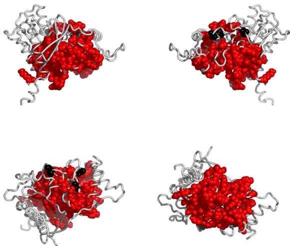
Fig. 4. Residues in IftaA, colored according to the cluster they belong to: red, followed by blue and yellow are the largest clusters (see Appendix for the coloring scheme). Clockwise: front, back, top and bottom views. The corresponding Pymol script is attached.
