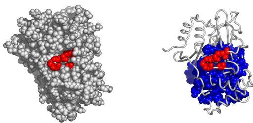
Fig. 8. Another possible active surface on the chain 1ftaA. The larger cluster it belongs to is shown in blue.
