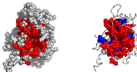
Fig. 7. A possible active surface on the chain 1ftaA. The larger cluster it belongs to is shown in blue.
