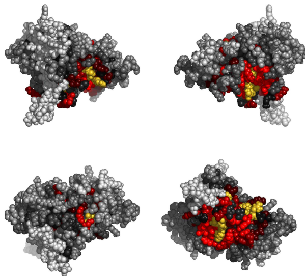
Fig. 3. Residues in IftaA, colored by their relative importance. Clockwise: front, back, top and bottom views.
