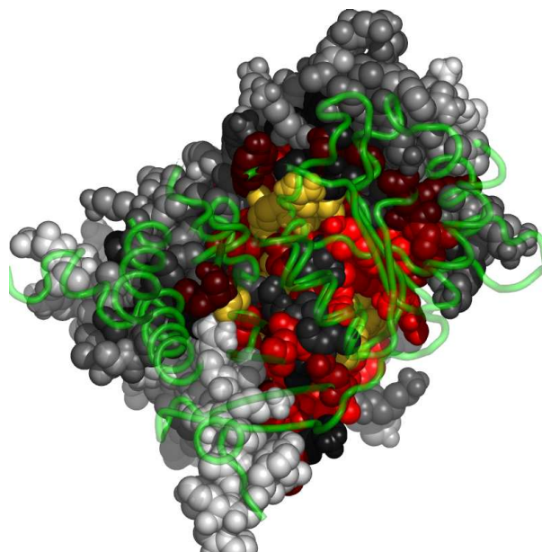
Fig. 5. Residues in 1ftaA, at the interface with 1ftaB, colored by their relative importance. 1ftaB is shown in backbone representation (See Appendix for the coloring scheme for the protein chain 1ftaA.)
