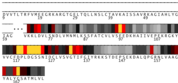
Fig. 1. Residues 9-175 in IftaA colored by their relative importance. (See Appendix, Fig.9, for the coloring scheme.)
