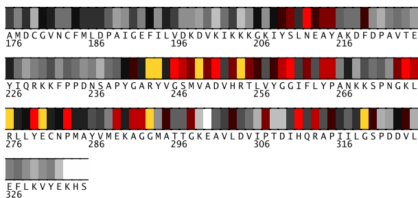
Fig. 2. Residues 176-335 in IftaA colored by their relative importance. (See Appendix, Fig.9, for the coloring scheme.)
