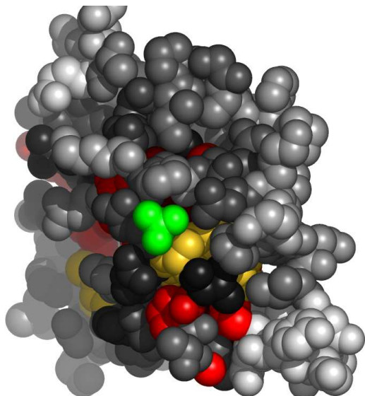
Fig. 6. Residues in 1fx9A, at the interface with sulfate ion, colored by their relative importance. The ligand (sulfate ion) is colored green. Atoms further than 30\text{\AA} away from the geometric center of the ligand, as well as on the line of sight to the ligand were removed. (See Appendix for the coloring scheme for the protein chain 1fx9A.)
