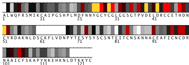
Fig. 1. Residues 1-124 in 1fx9A colored by their relative importance. (See Appendix, Fig.7, for the coloring scheme.)
