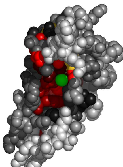
Fig. 5. Residues in 1fx9A, at the interface with calcium ion, colored by their relative importance. The ligand (calcium ion) is colored green. Atoms further than 30Å away from the geometric center of the ligand, as well as on the line of sight to the ligand were removed. (See Appendix for the coloring scheme for the protein chain 1fx9A.)
