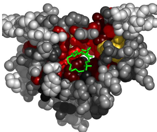
Fig. 4. Residues in 1fx9A, at the interface with MJI, colored by their relative importance. The ligand (MJI) is colored green. Atoms further than 30Å away from the geometric center of the ligand, as well as on the line of sight to the ligand were removed. (See Appendix for the coloring scheme for the protein chain 1fx9A.)
