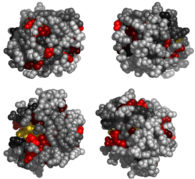
Fig. 2. Residues in 1g2iA, colored by their relative importance. Clockwise: front, back, top and bottom views.
