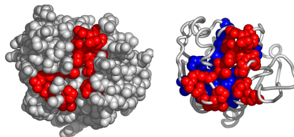
Fig. 7. A possible active surface on the chain 1g2iA. The larger cluster it belongs to is shown in blue.
