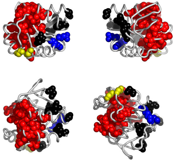
Fig. 3. Residues in 1g2iA, colored according to the cluster they belong to: red, followed by blue and yellow are the largest clusters (see Appendix for the coloring scheme). Clockwise: front, back, top and bottom views. The corresponding Pymol script is attached.
