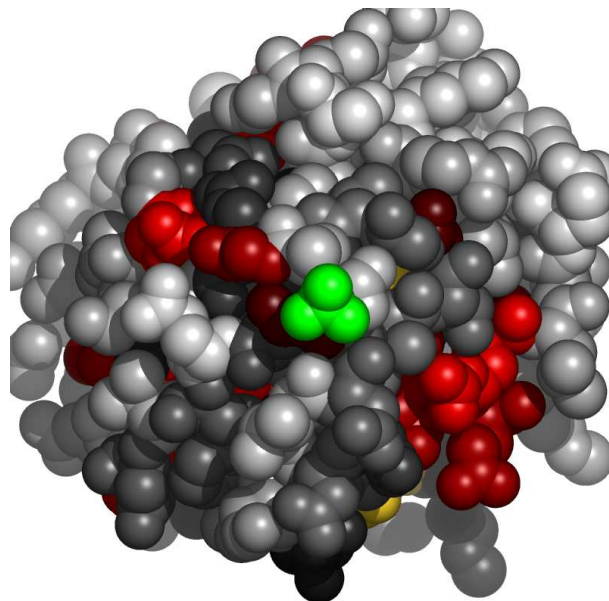
Fig. 6. Residues in 1g2iA, at the interface with sulfate ion, colored by their relative importance. The ligand (sulfate ion) is colored green. Atoms further than 30Å away from the geometric center of the ligand, as well as on the line of sight to the ligand were removed. (See Appendix for the coloring scheme for the protein chain 1g2iA.)
