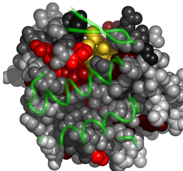
Fig. 5. Residues in 1g2iA, at the interface with 1g2iB, colored by their relative importance. 1g2iB is shown in backbone representation (See Appendix for the coloring scheme for the protein chain 1g2iA.)
