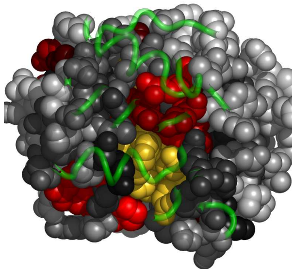
Fig. 4. Residues in 1g2iA, at the interface with 1g2iC, colored by their relative importance. 1g2iC is shown in backbone representation (See Appendix for the coloring scheme for the protein chain 1g2iA.)
