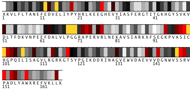
Fig. 1. Residues 1-166 in 1g2iA colored by their relative importance. (See Appendix, Fig.8, for the coloring scheme.)
