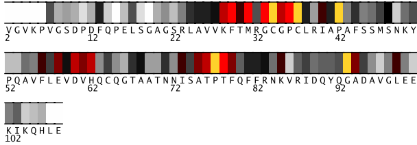
Fig. 1. Residues 2-108 in 1gh2A colored by their relative importance. (See Appendix, Fig.5, for the coloring scheme.)
