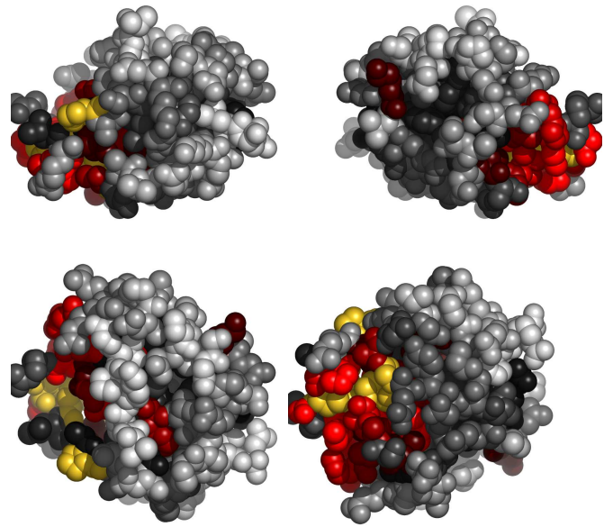
Fig. 2. Residues in 1gh2A, colored by their relative importance. Clockwise: front, back, top and bottom views.
