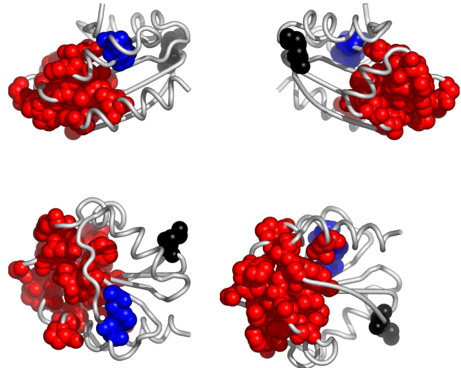
Fig. 3. Residues in 1gh2A, colored according to the cluster they belong to: red, followed by blue and yellow are the largest clusters (see Appendix for the coloring scheme). Clockwise: front, back, top and bottom views. The corresponding Pymol script is attached.
