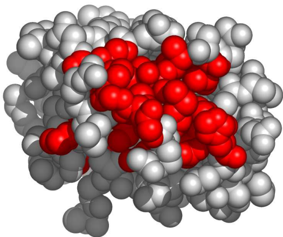
Fig. 4. A possible active surface on the chain 1gh2A.
