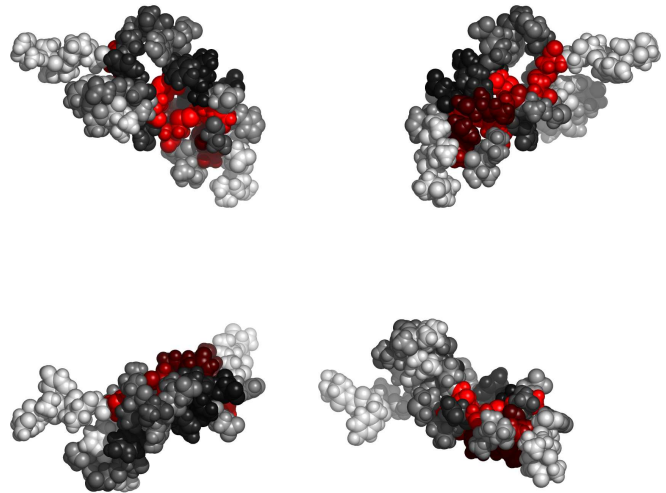
Fig. 1. Residues 1-49 in 1gk5A colored by their relative importance. (See Appendix, Fig.5, for the coloring scheme.)
