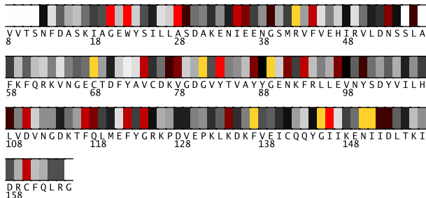
Fig. 1. Residues 8-165 in 1gm6A colored by their relative importance. (See Appendix, Fig.8, for the coloring scheme.)
