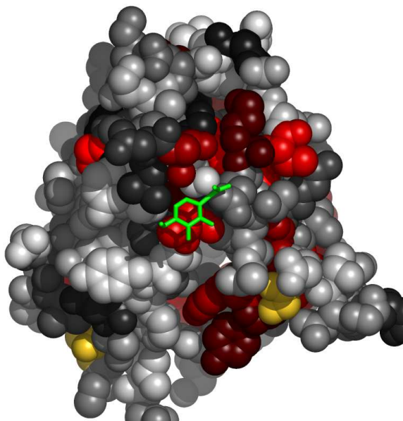
Fig. 5. Residues in 1gm6A, at the interface with NAG, colored by their relative importance. The ligand (NAG) is colored green. Atoms further than 30Å away from the geometric center of the ligand, as well as on the line of sight to the ligand were removed. (See Appendix for the coloring scheme for the protein chain 1gm6A.)
