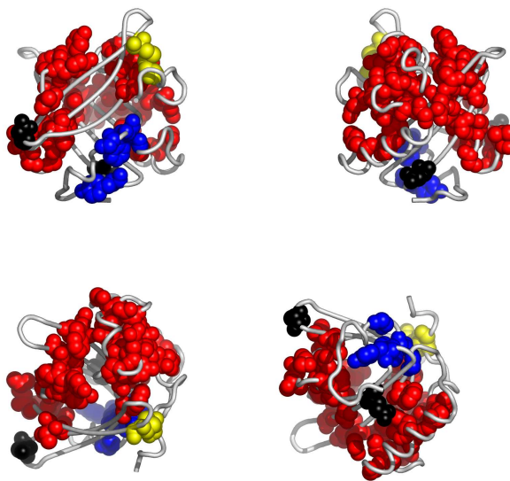
Fig. 3. Residues in 1gm6A, colored according to the cluster they belong to: red, followed by blue and yellow are the largest clusters (see Appendix for the coloring scheme). Clockwise: front, back, top and bottom views. The corresponding Pymol script is attached.
