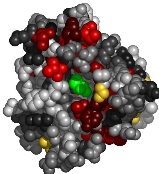
Fig. 4. Residues in 1gm6A, at the interface with glycerol, colored by their relative importance. The ligand (glycerol) is colored green. Atoms further than 30Å away from the geometric center of the ligand, as well as on the line of sight to the ligand were removed. (See Appendix for the coloring scheme for the protein chain 1gm6A.)
