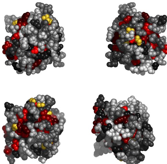
Fig. 2. Residues in 1gm6A, colored by their relative importance. Clockwise: front, back, top and bottom views.
