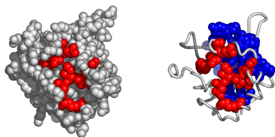
Fig. 7. Another possible active surface on the chain 1gm6A. The larger cluster it belongs to is shown in blue.
