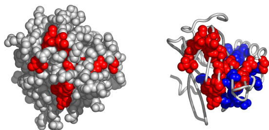
Fig. 6. A possible active surface on the chain 1gm6A. The larger cluster it belongs to is shown in blue.
